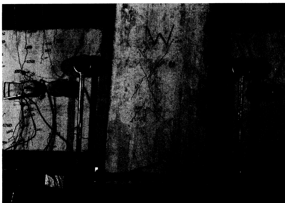
Fig. 20—M-P-Z4 at failure (3.4 percent story drift)
