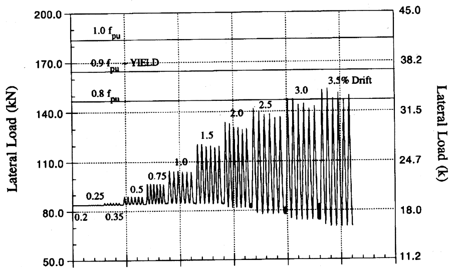
Fig. 25—Typical force in prestressing strand, M-P-Z4
