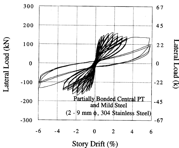
Fig. 28—Hysteresis curves for N-P-Z4
