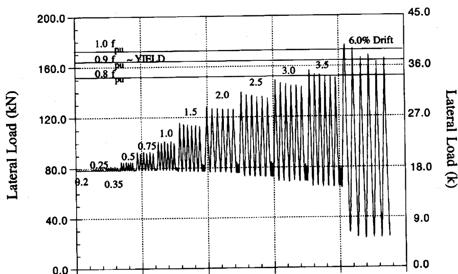
Fig. 26—Typical force in prestressing strand, N-P-Z4
