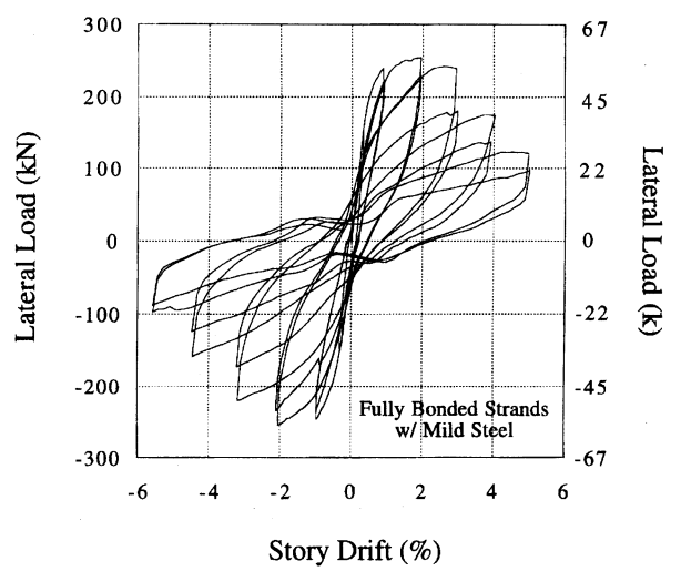
Fig. 12—Hysteresis curves for K-P-Z4
