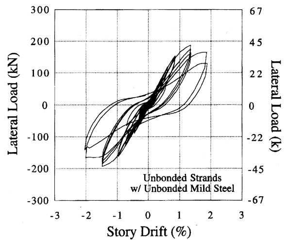
Fig. 13—Hysteresis curves for L-P-Z4 C
