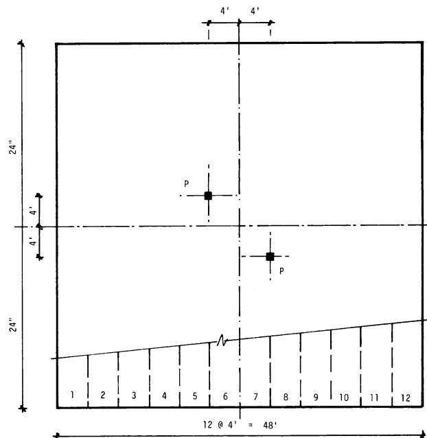
Fig. 16 — Deck for Example 4
