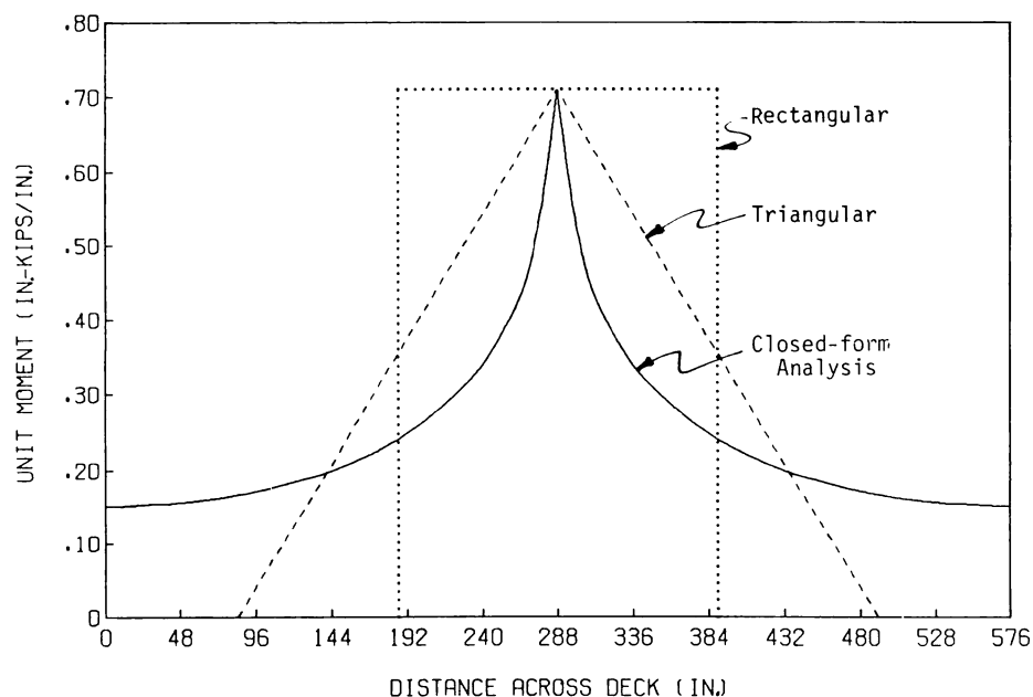
Fig. 1 — Lateral variation of unit longitudinal bending moment
