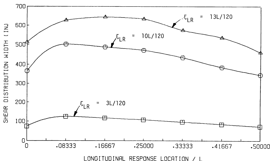
Fig. 9 — Variation of distribution width for longitudinal shear with longitudinal response location
