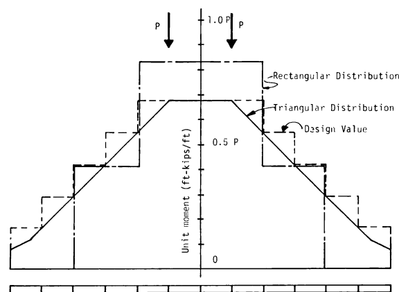
Fig. 17 — Transverse variation on unit moment in Example 4
