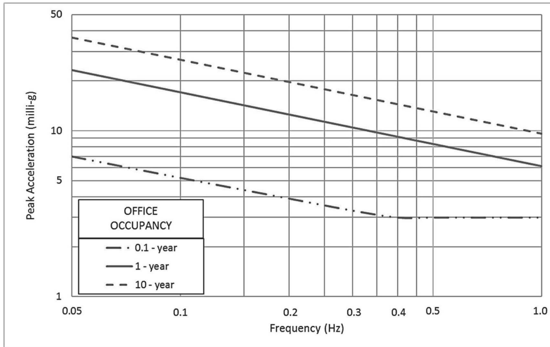
(a) Comfort criteria for office occupancy buildings.
