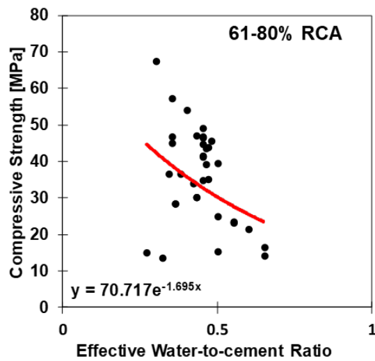
Fig. 6- Variation of RCA compressive strength with effective water-to-cement ratio
