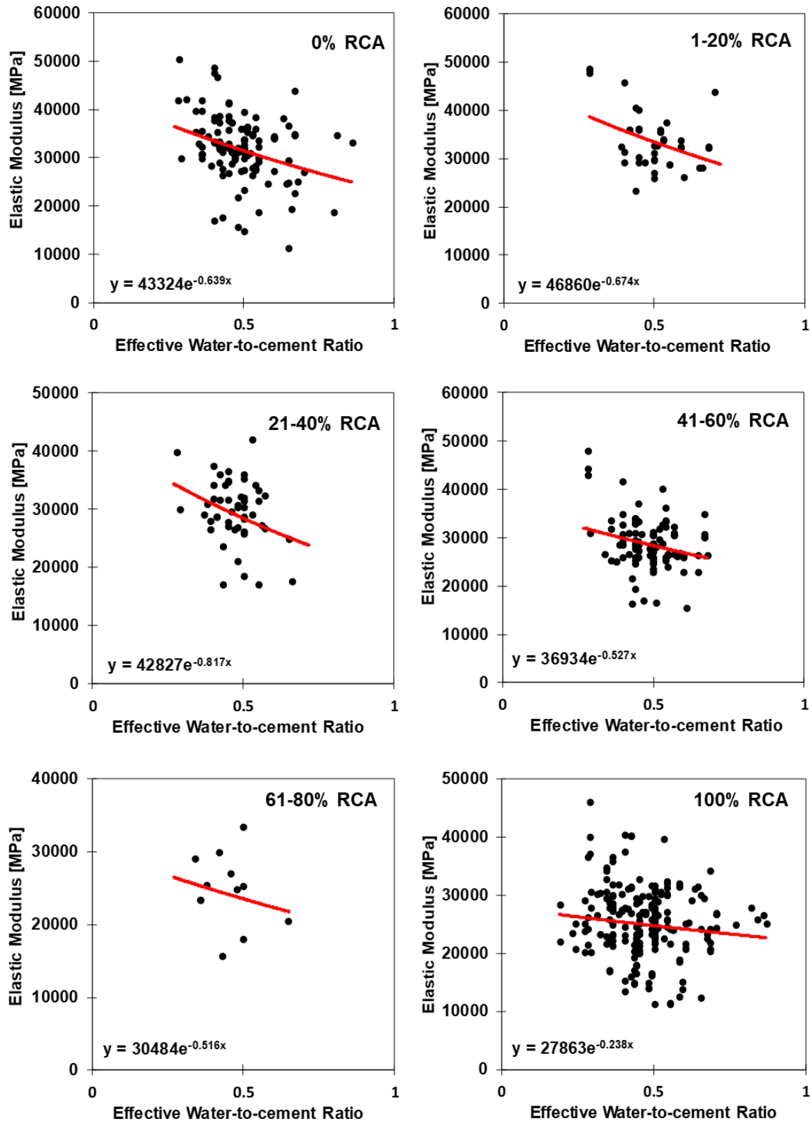
Fig. 8- Variation of RCA elastic modulus with effective water-to-cement ratio
