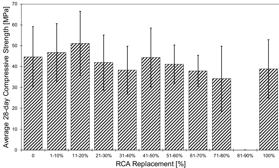
Fig. 4- Mean compressive strength variation of RAC systems over RCA replacement levels
