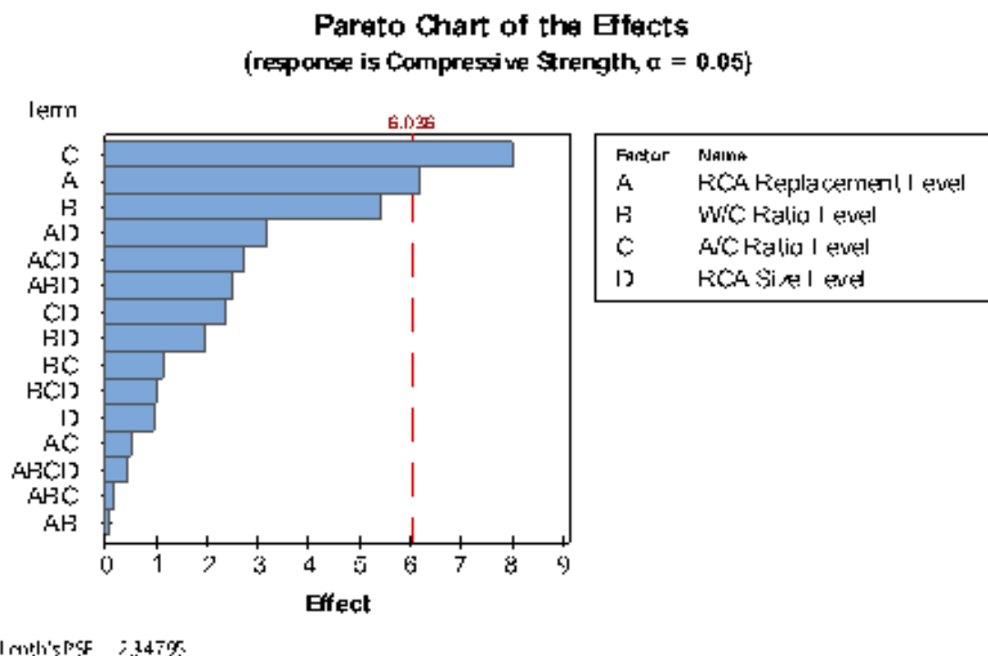
Fig. 14- Pareto chart of the standardized effects at 95% confidence interval on compressive strength
