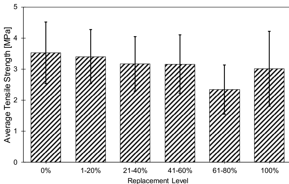
Fig. 9- Mean splitting tensile strength variation of RAC systems over RCA replacement levels
