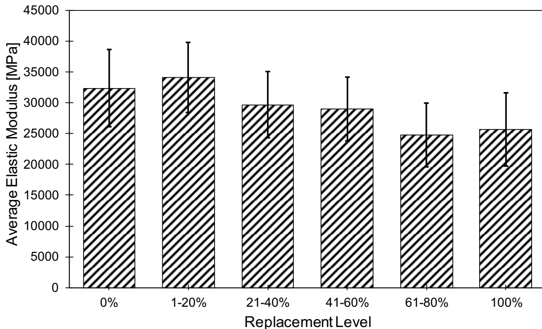
Fig. 7- Mean elastic modulus variation of RAC systems over RCA replacement levels
