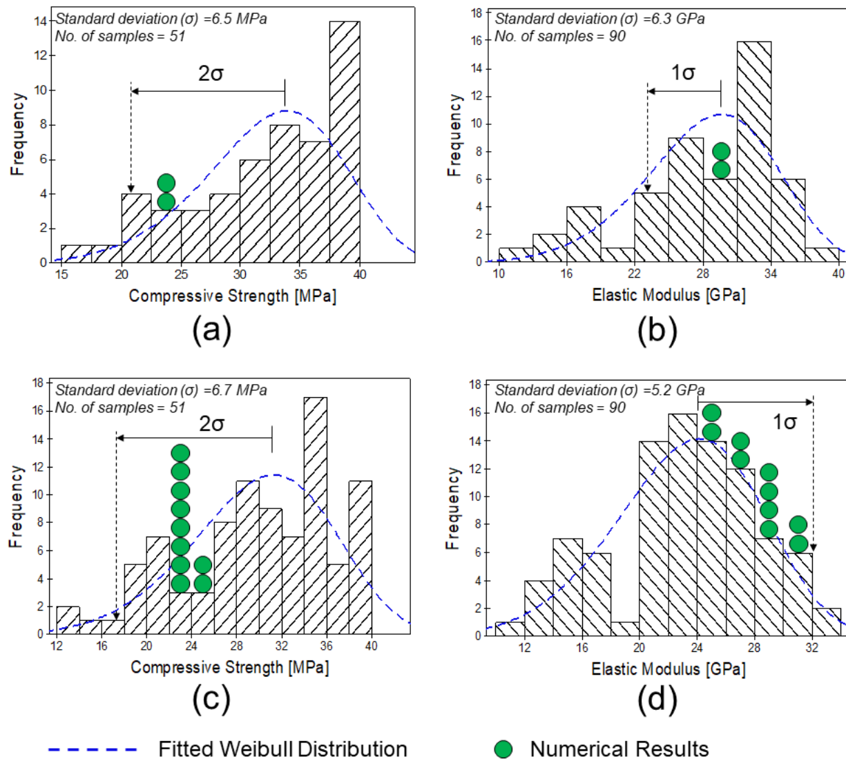
Fig. 19- Histogram of the material properties of two systems; (a) compressive strength for 0% replacement level (b) elastic modulus for 0% replacement level (c) compressive strength for 100% replacement level (d) elastic modulus for 100% replacement level
