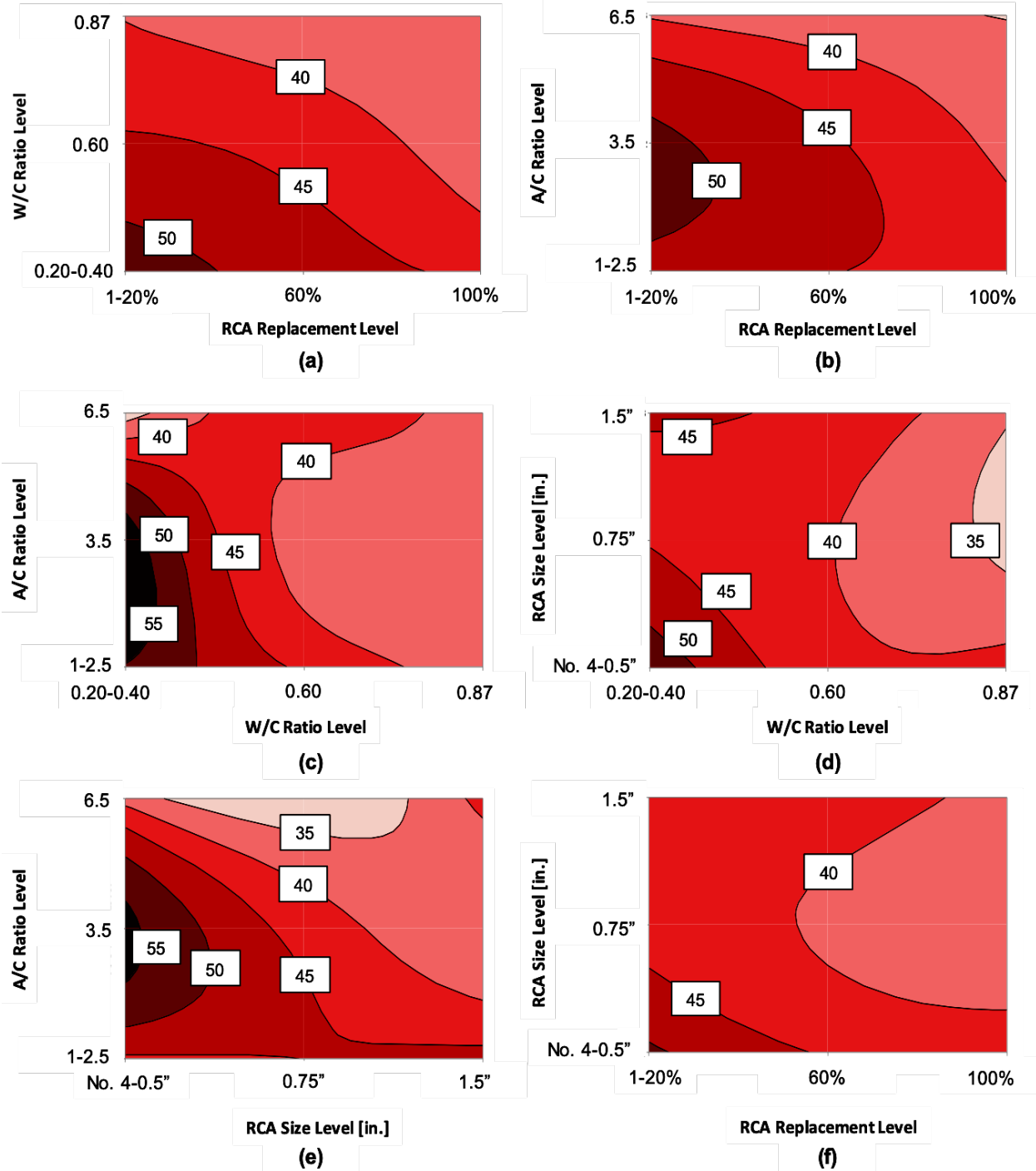
Fig. 16- Bi-variate relationships generated for RCA compressive strengths in MPa
