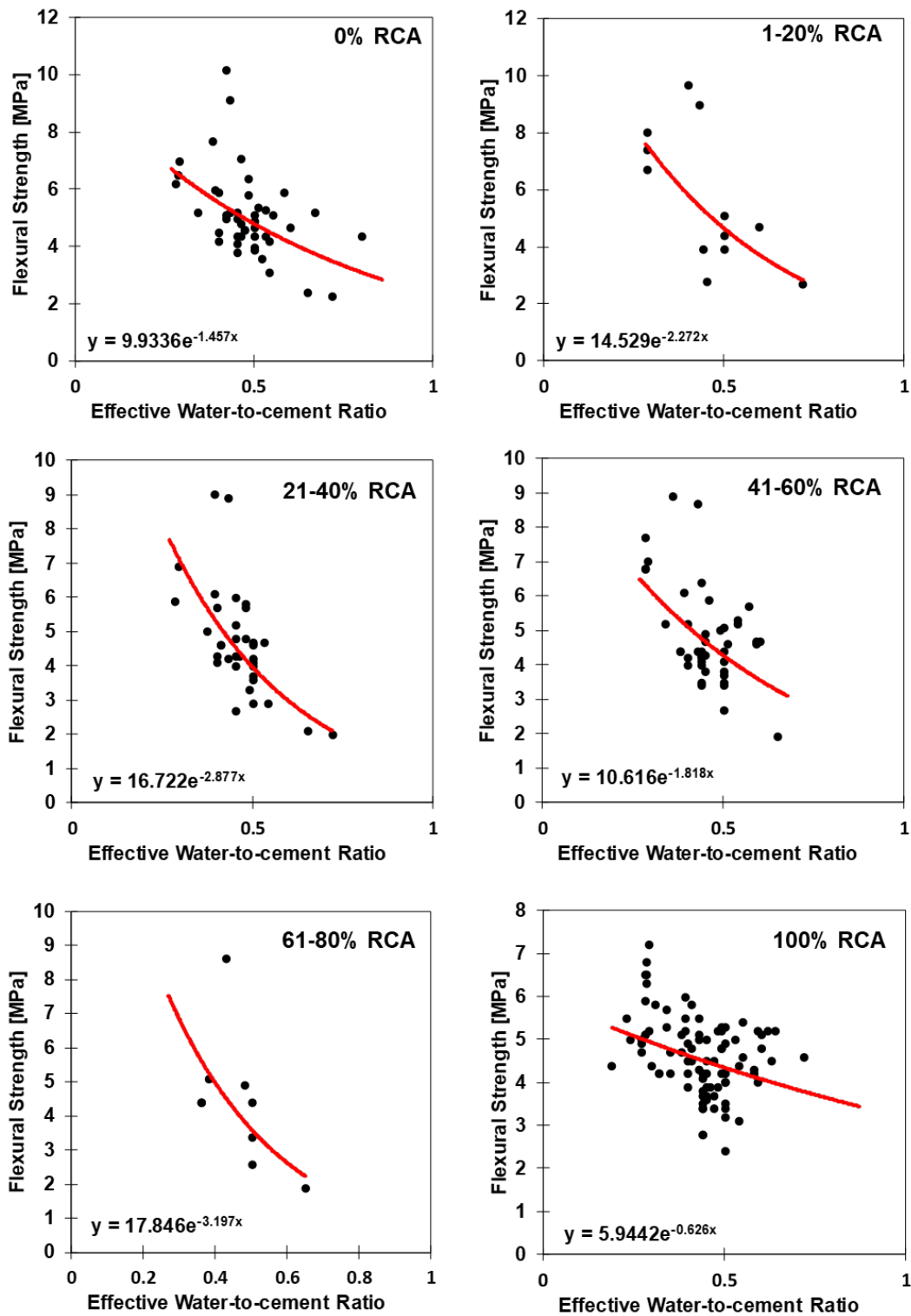
Fig. 12- Variation of RCA flexural strength with effective water-to-cement ratio
