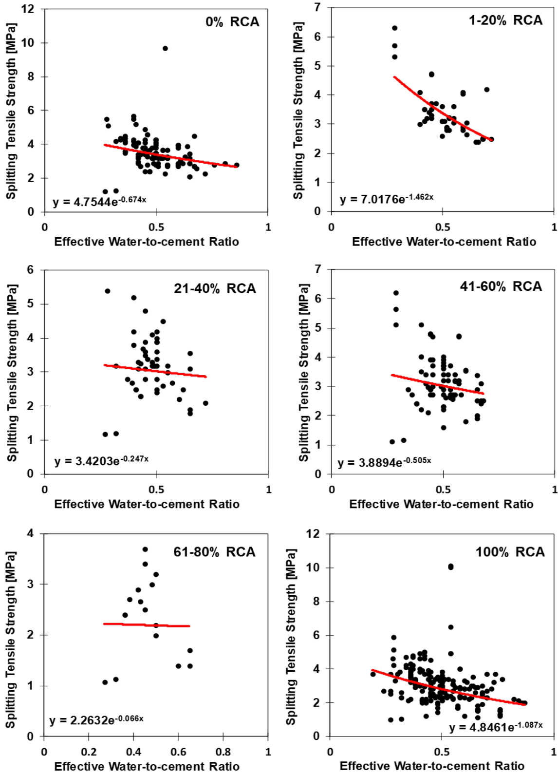
Fig. 10- Variation of RCA splitting tensile strength with effective water-to-cement ratio
