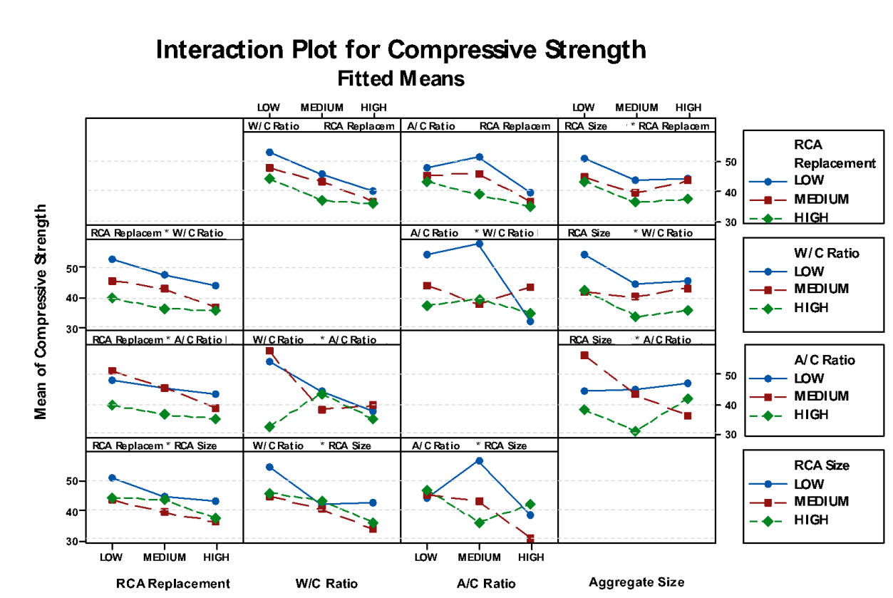
Fig. 15- Interaction plot matrix
