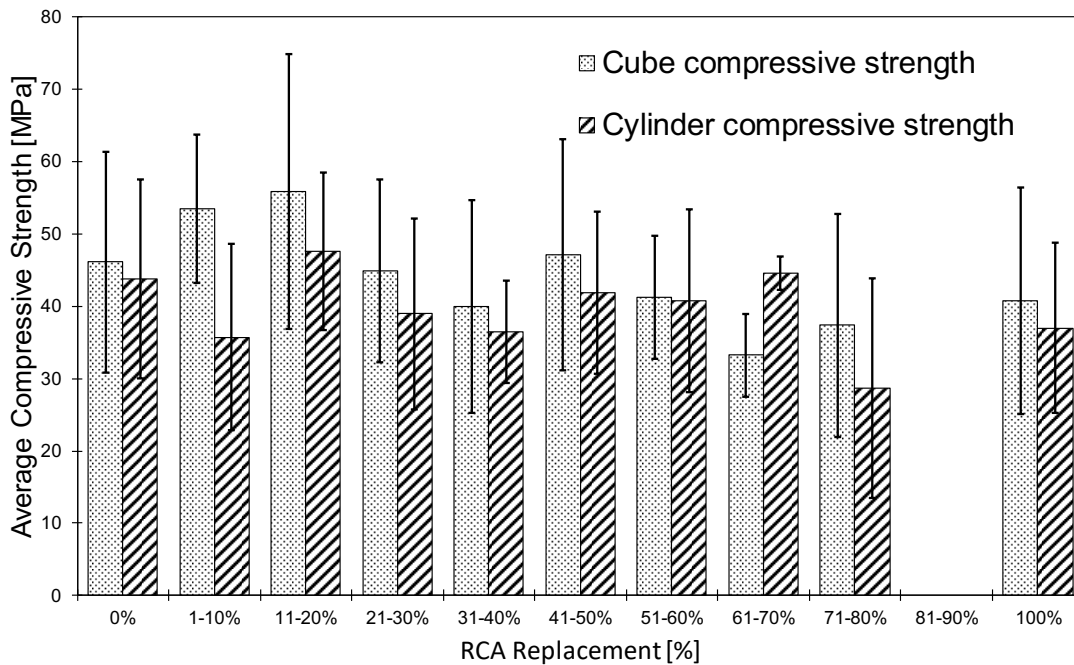
Fig. 5- Comparison of compressive strength cast from two different specimen types
