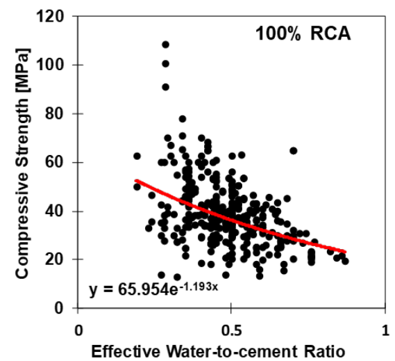
Fig. 6- Variation of RCA compressive strength with effective water-to-cement ratio
