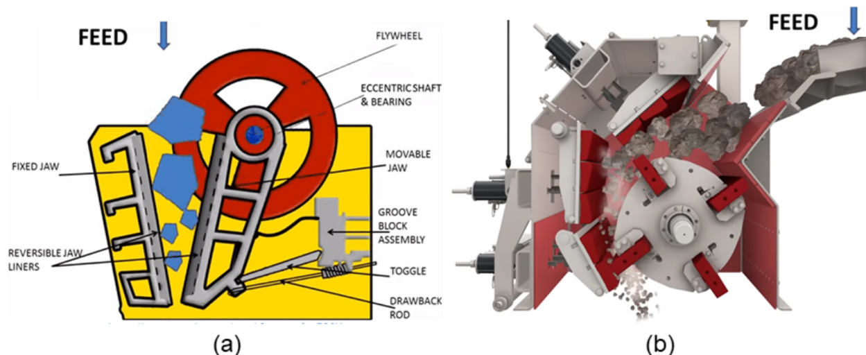
Fig. 2- RCA crusher types; (a) jaw-type crusher 31 (b) impact crusher 32
