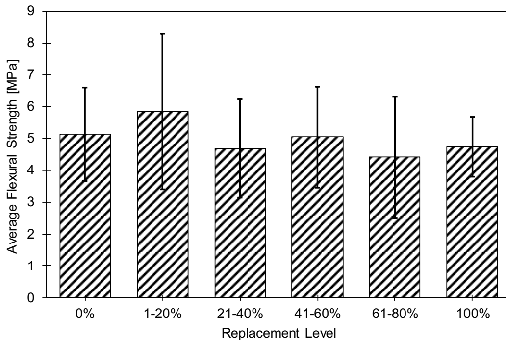
Fig. 11- Mean flexural strength variation of RAC systems over RCA replacement levels
