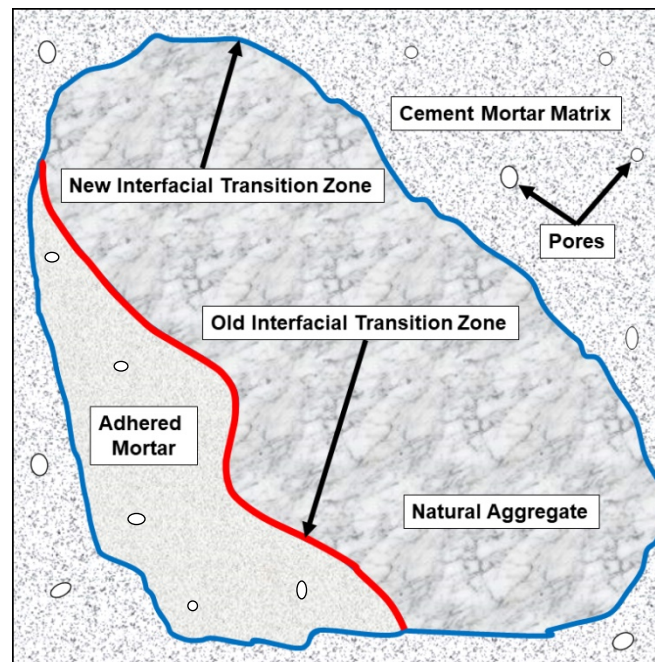
Fig. 1- Meso-scale material phases in RCA concrete systems
