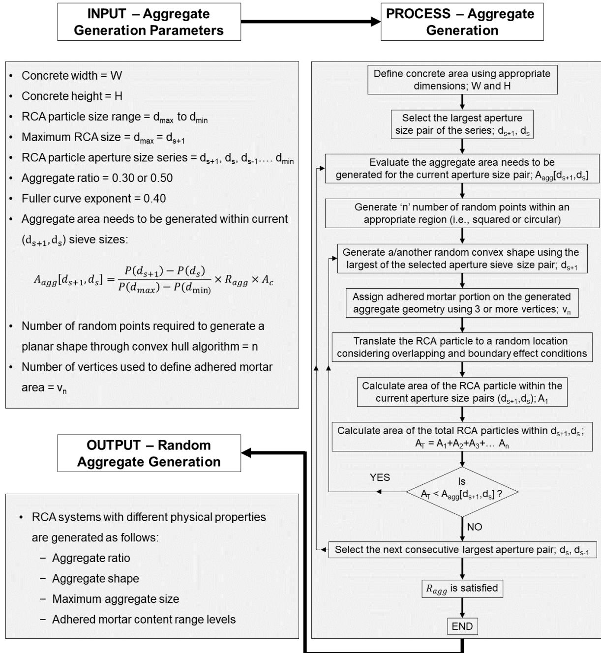
Fig. 17- Aggregate generation process flow chart
