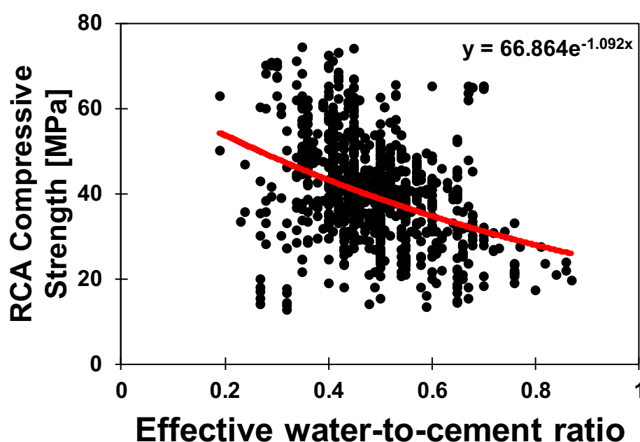
Fig. 20- Compressive strength trend over the effective water-to-cement ratio after eliminating possible outliers
