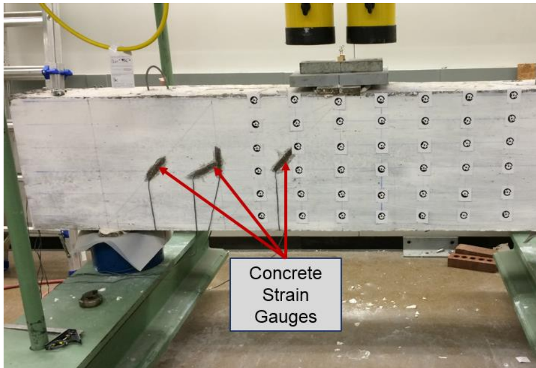
Figure 3-17: Example of Concrete Strain Gauges on Beam
