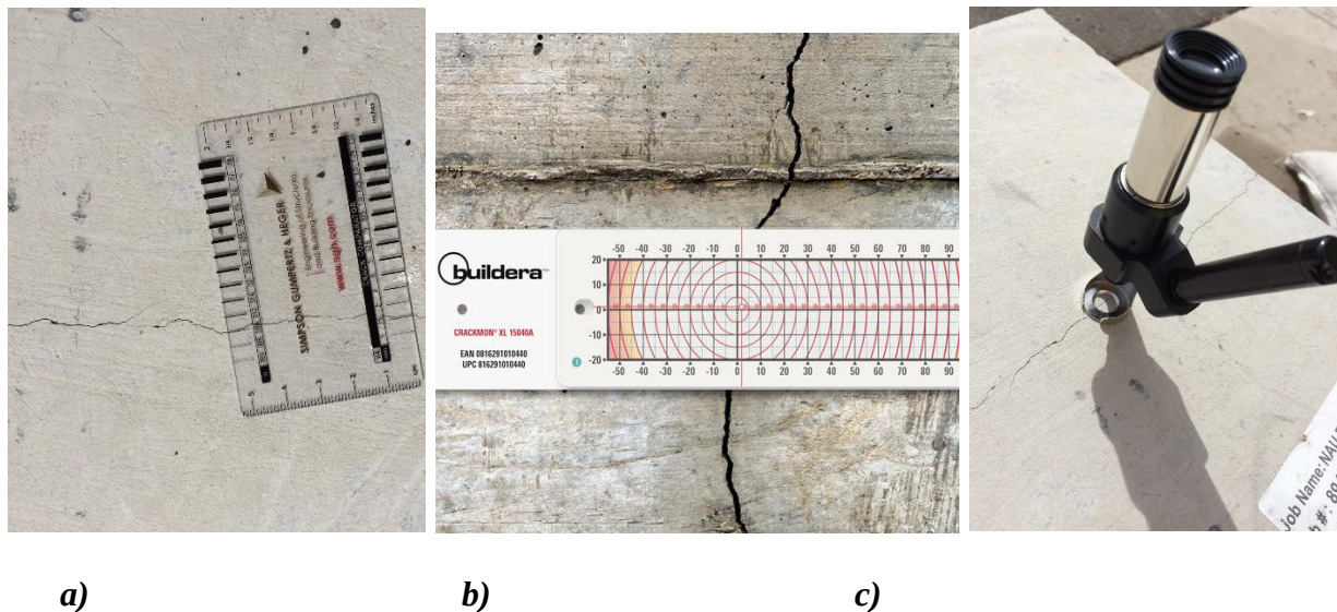
Figure 2-18: a) Crack comparator card; b) Calipers and; c) Microscope
