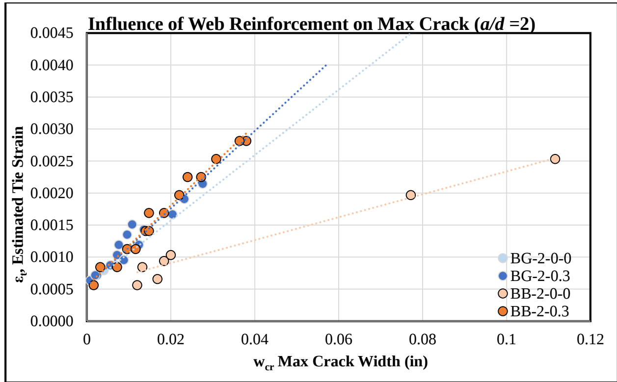
Figure 5-2: Influence of Web Reinforcement on Max Crack ( a/d = 2 )
