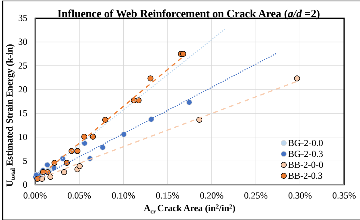
Figure 5-7: Influence of Web Reinforcement on Crack Area ( a/d = 2 )
