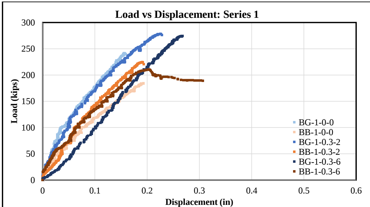
Figure 4-1: Series 1 Load vs. Displacement Data
