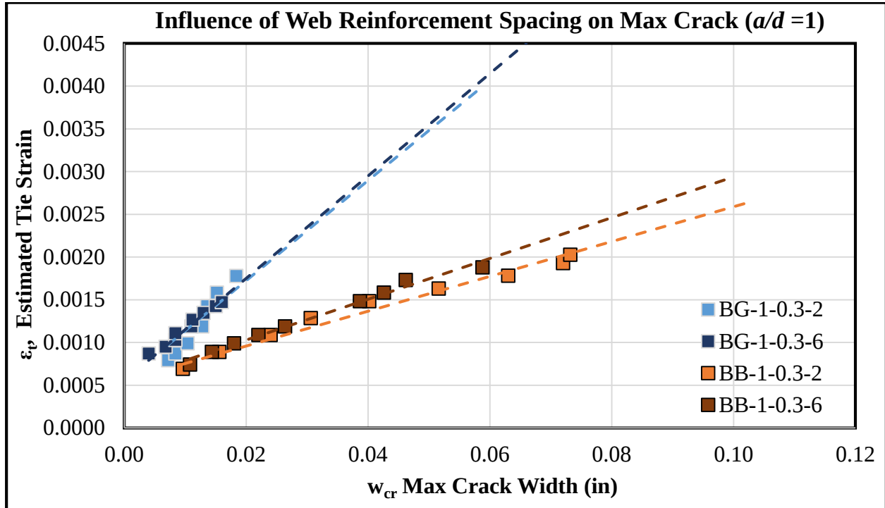
Figure 5-3: Influence of Web Reinforcement Spacing on Max Crack ( a/d = 1 )
