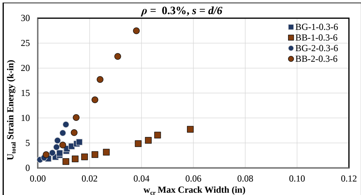
Figure 4-13: Max Diagonal Crack Width vs. Total Strain Energy for \rho = 0.3\% , s = d/6
