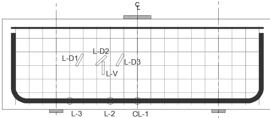
Figure 4-6: BG-2-0.3-6 Steel and Concrete Gauge Locations
