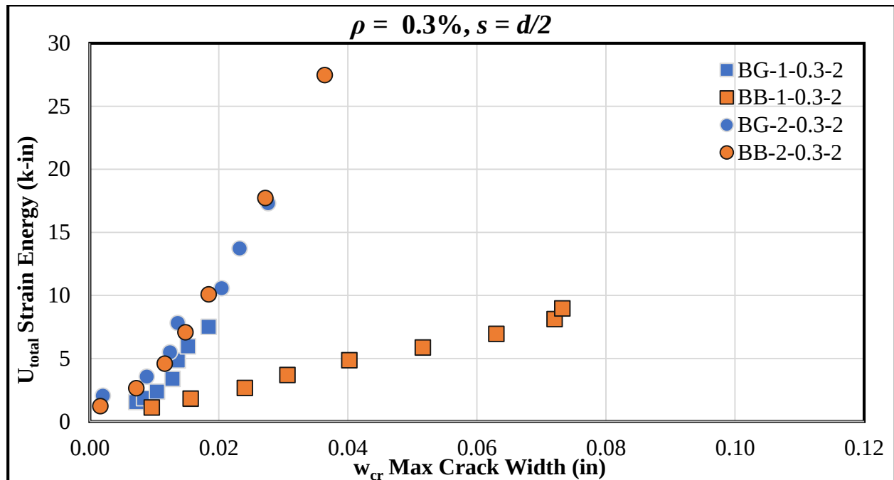
Figure 4-12: Max Diagonal Crack Width vs. Total Strain Energy for \rho = 0.3\% , s = d/2
