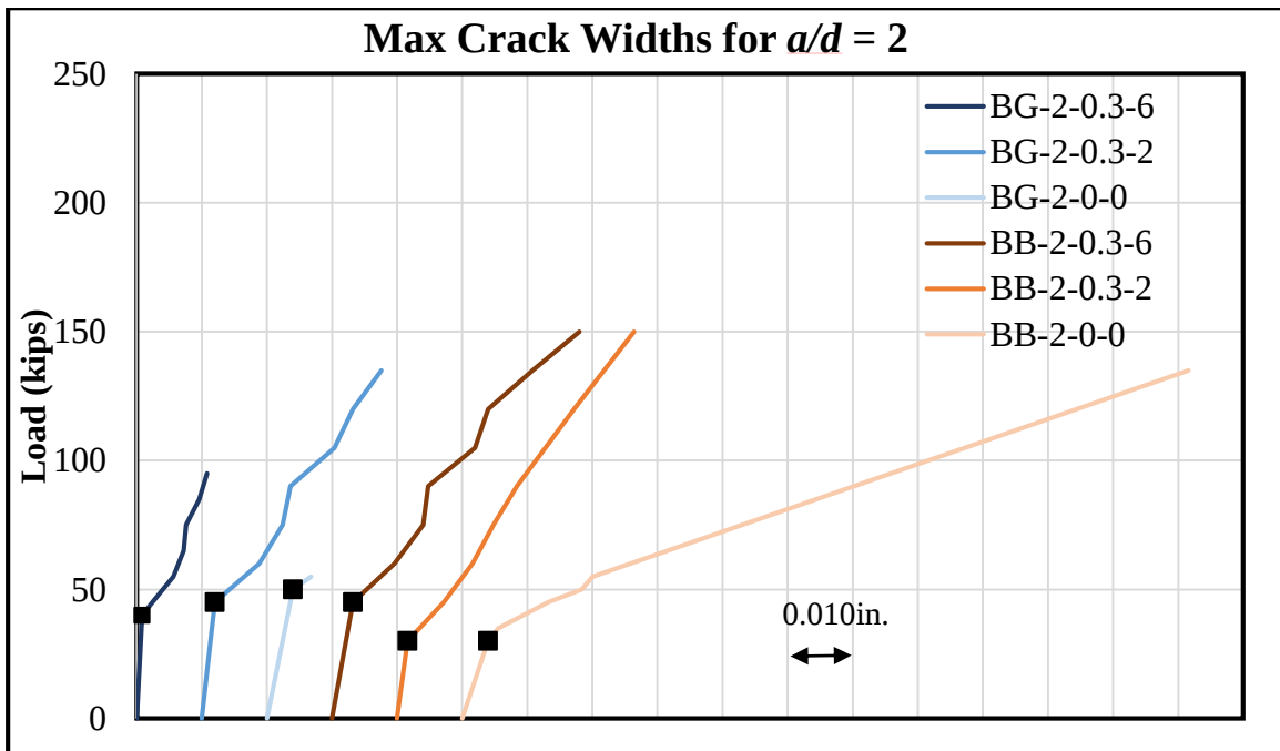
Figure 4-10: Maximum Crack Widths for Series 2 Specimens
