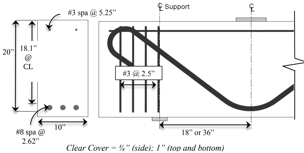
Figure 3-5: Specimens BB-1-0-0 & BB-2-0-0
