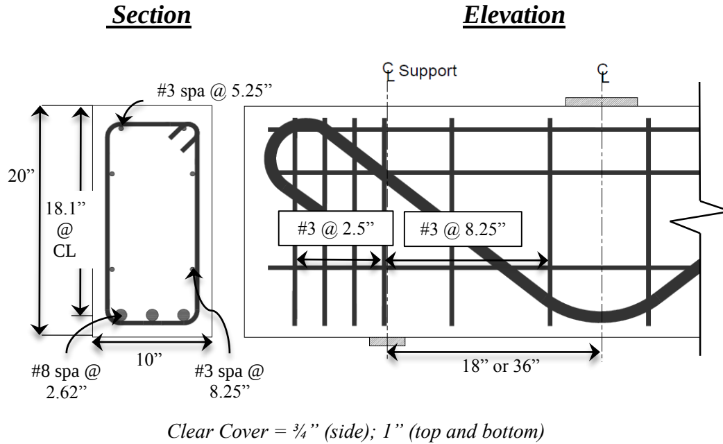
Figure 3-6: Specimens BB-1-0.3-2 & BB-2-0.3-2
