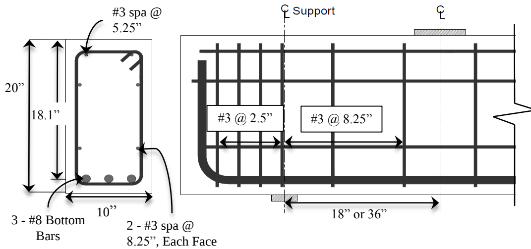
Figure 3-3: Specimen BG-1-0.3-2 & BG-2-0.3-2
