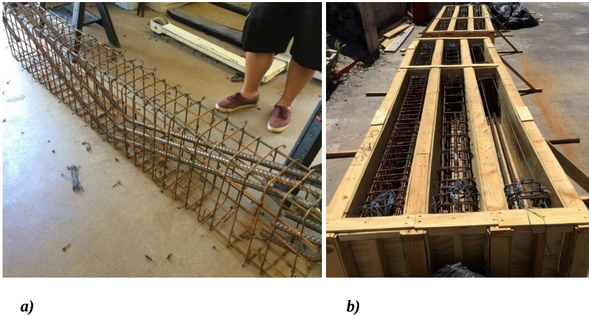
Figure 3-12: a) Rebar Cage for BB-2-0.3-6 and b) Assembled Cages in Formwork
