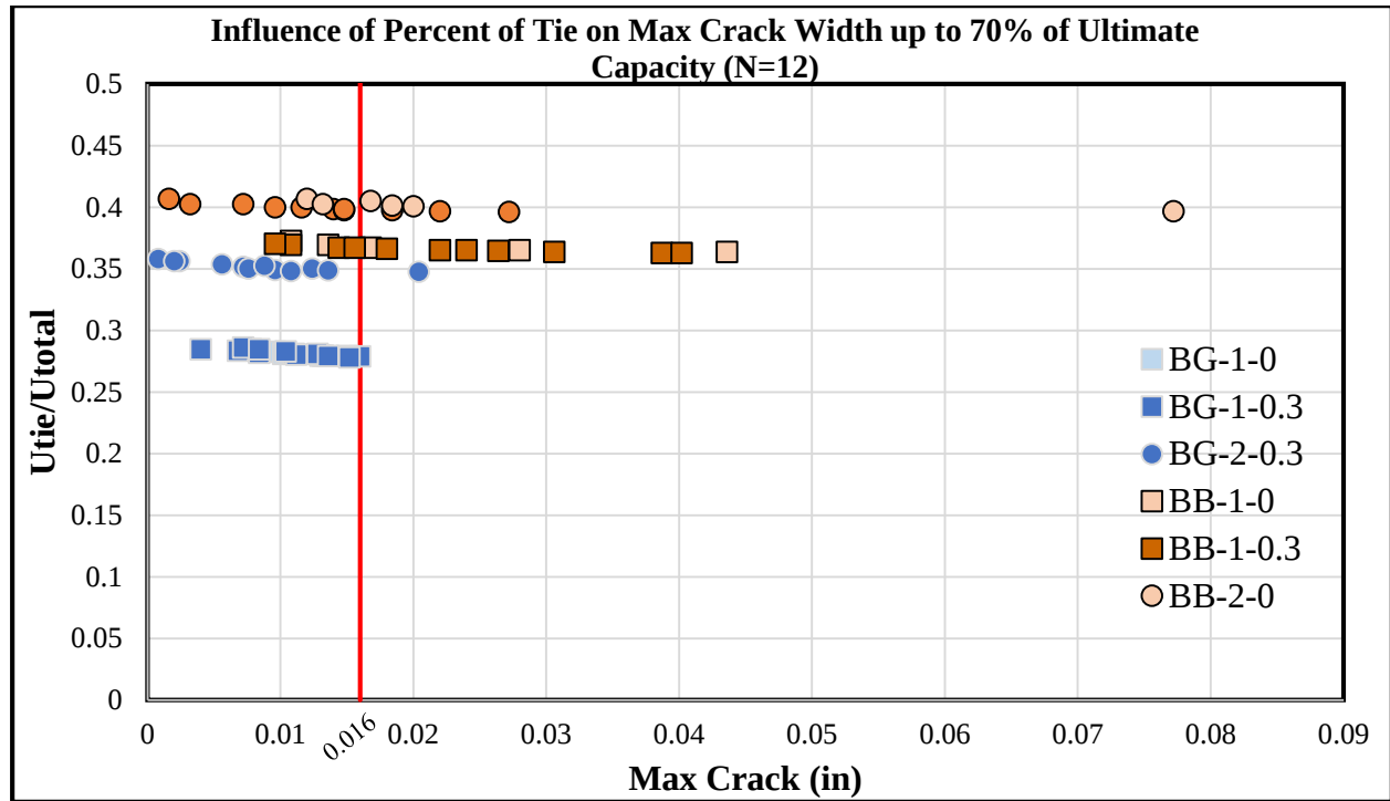
Figure 5-15: U_{tie}/U_{total} versus Maximum Crack Width up to 70% of ultimate capacity
