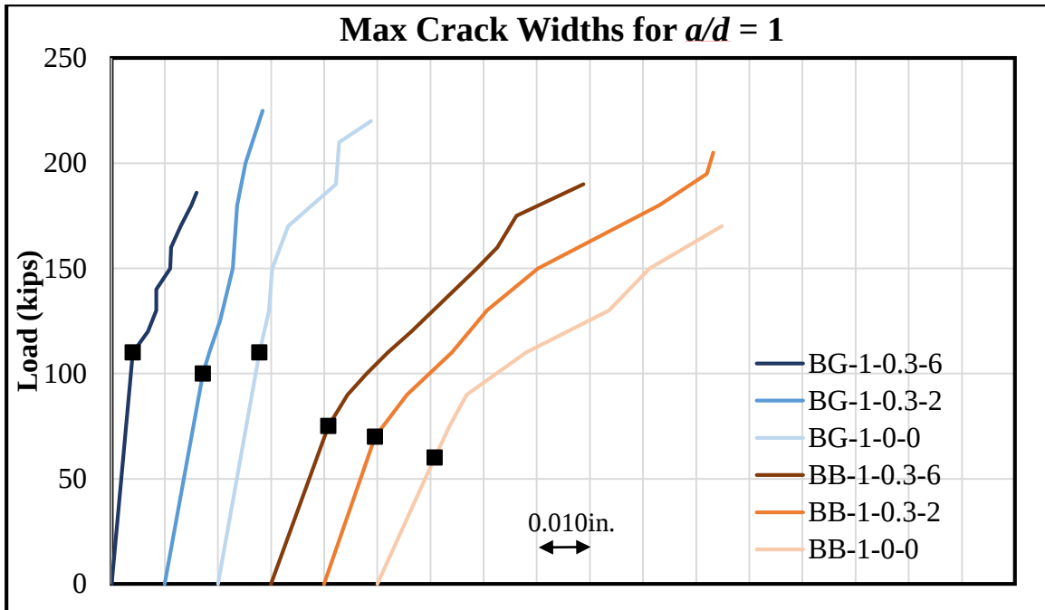
Figure 4-9: Maximum Crack Widths for Series 1 Specimens
