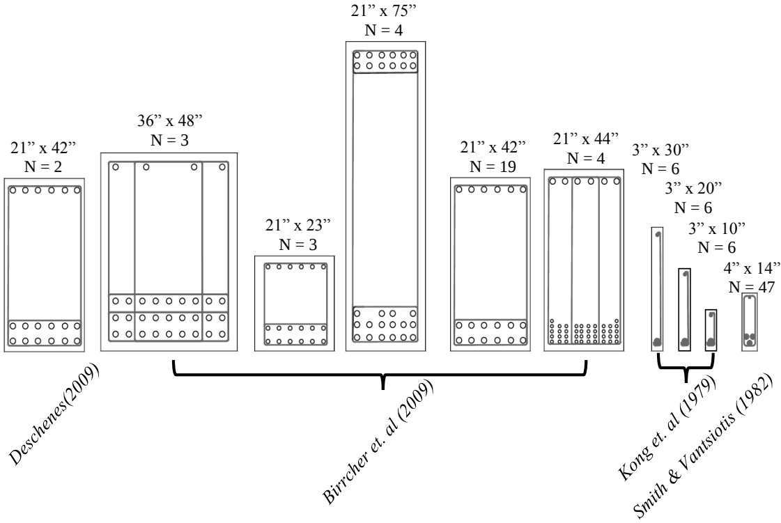
Figure 2-16: Cross-sectional dimensions and number of beams in the database
