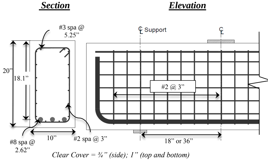
Figure 3-4: Specimens BG-1-0.3-6 & BG-2-0.3-6
