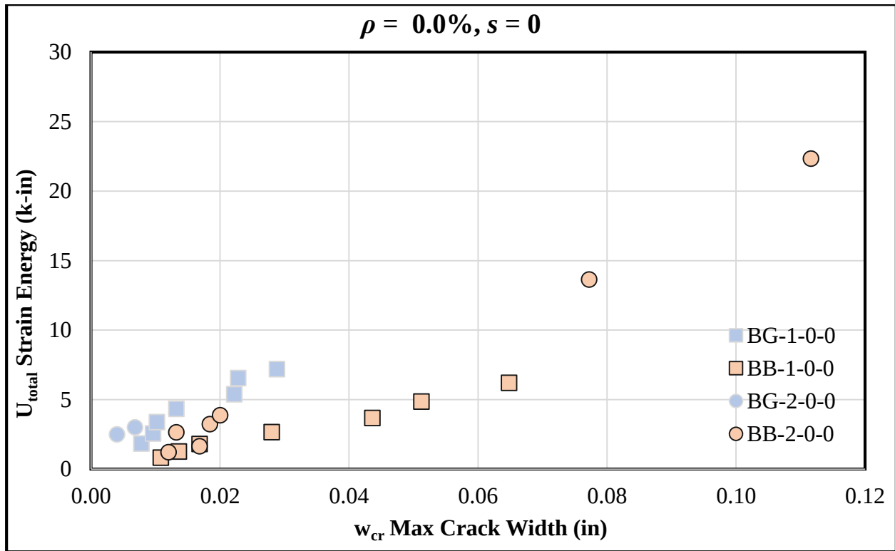
Figure 4-11: Max Diagonal Crack Width vs. Strain Energy for \rho = 0.0\% , s = 0
