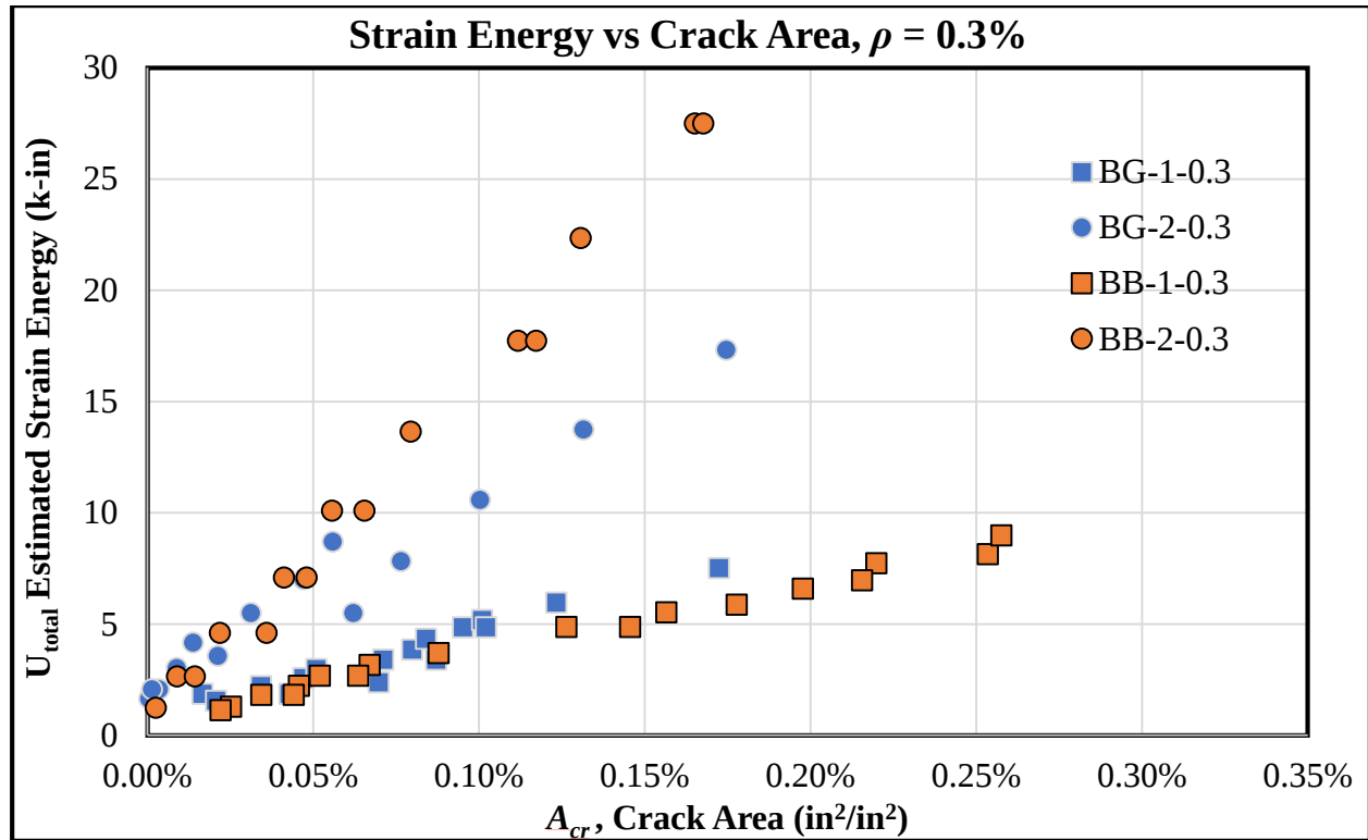
Figure 5-14: Relationship between Strain Energy and Crack Area
