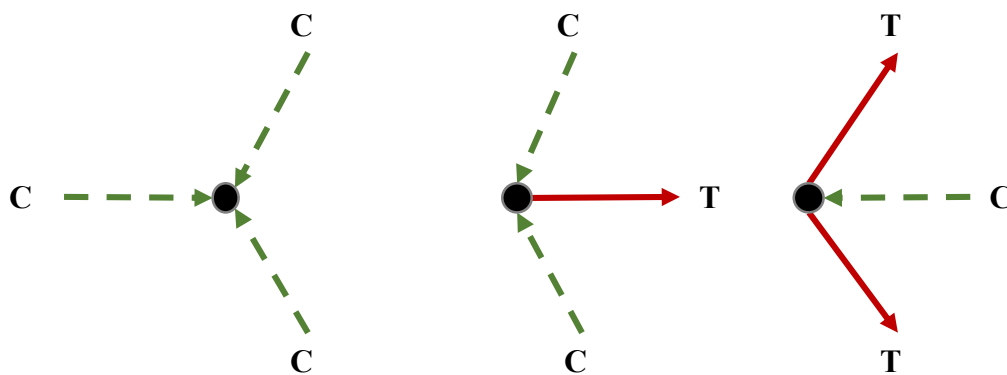
Figure 2-8: Classification of Nodes (ACI 318-14)
