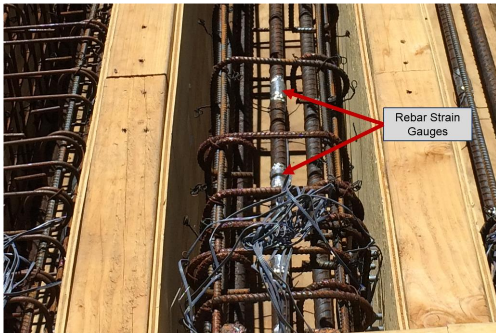
Figure 3-16: Rebar Strain Gauges
