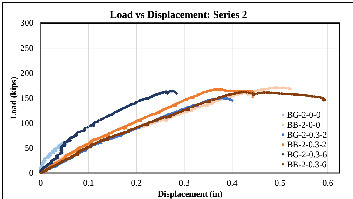
Figure 4-2: Series 2 Load vs. Displacement Data
