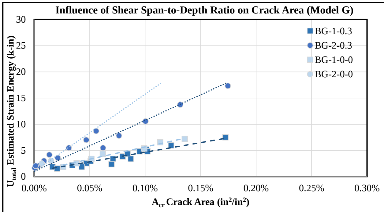
Figure 5-11: Influence on Shear Span-to-Depth Ratio on Crack Area (Model G)
