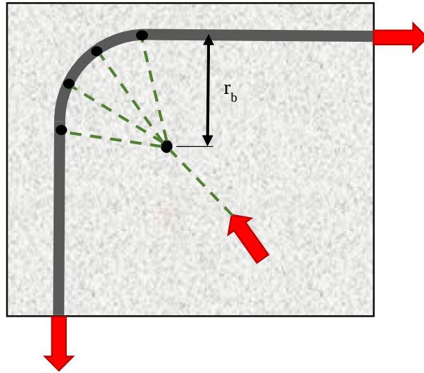
Figure 2-13: Curved Bar CTT Node
