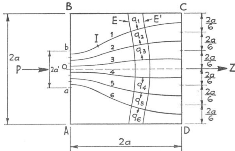
Figure 2-6: Dispersion of Compressive Stress (Guyon 1953)
