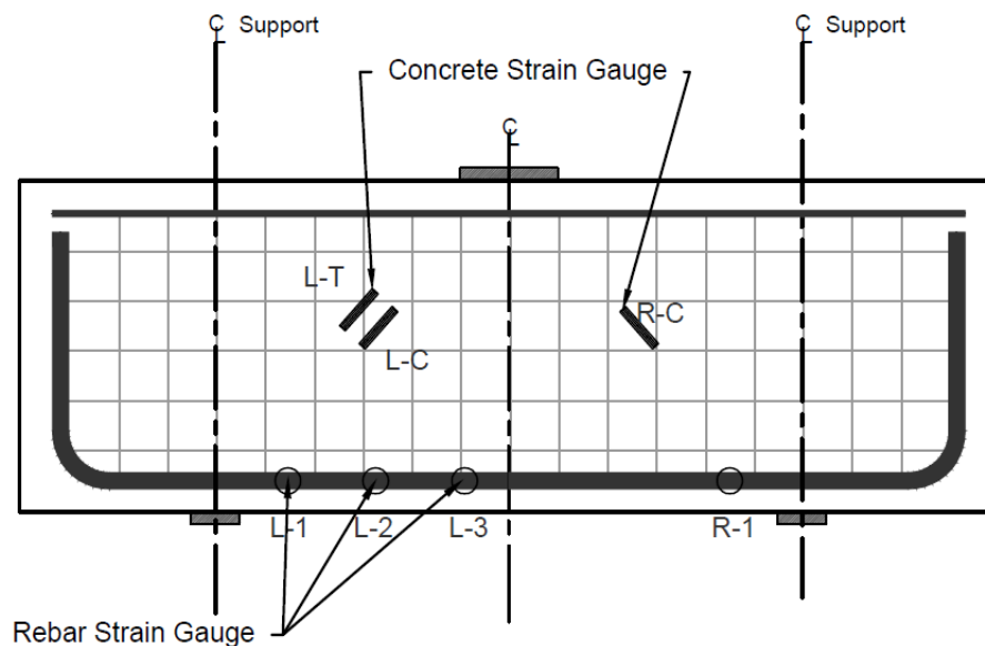
Figure 3-15: Strain Gauge Locations for BG-1-0.3-6
