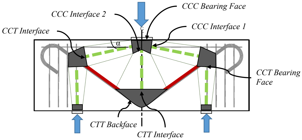
Figure 3-10: Model B Nodal Geometry
