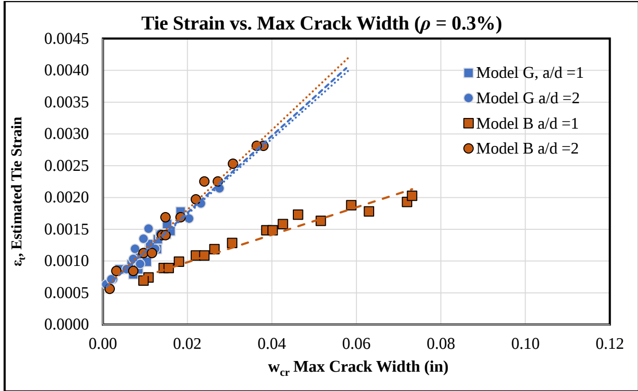
Figure 5-13: Relationship of Tie Strain and Maximum Crack Width ( \rho = 0.3\% )
