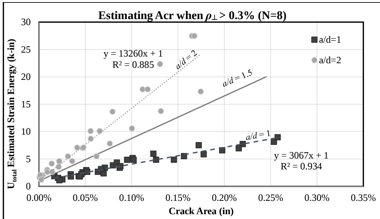
Figure 5-17: Design Tool for Predicting Crack Area
