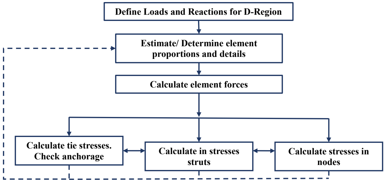
Figure 2-10: Strut and Tie Design Flowchart
