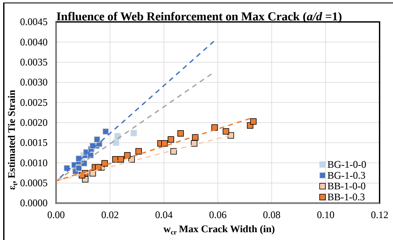
Figure 5-1: Influence of Web Reinforcement on Max Crack ( a/d = 1 )
