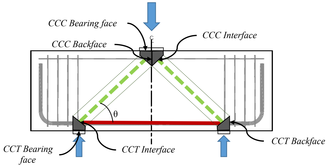
Figure 3-9: Model G Node Locations
