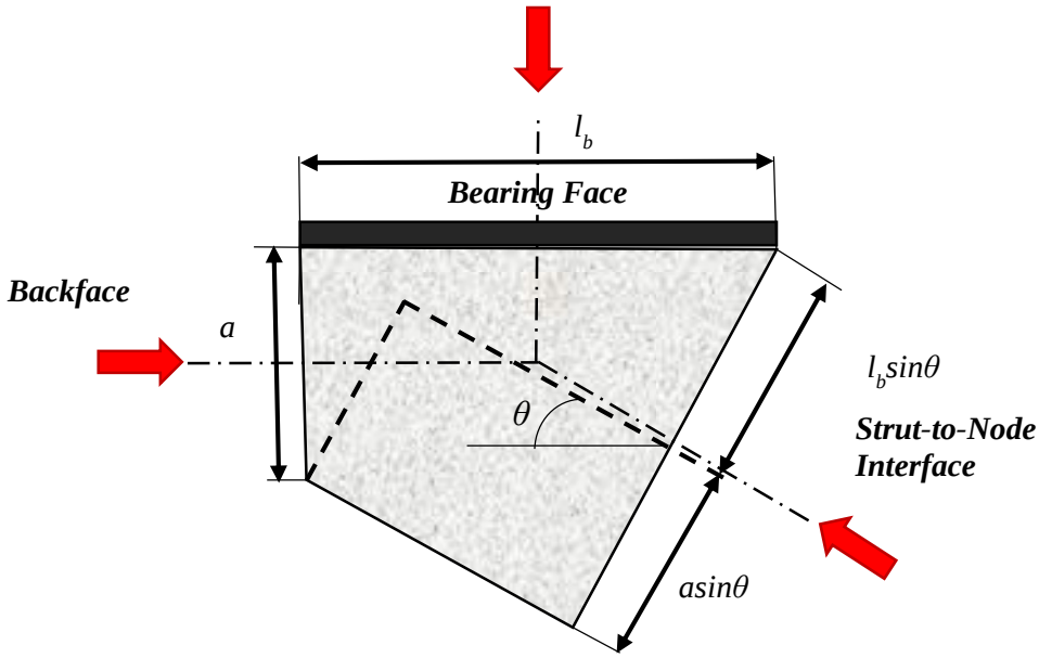
Figure 2-12: CCC Node
