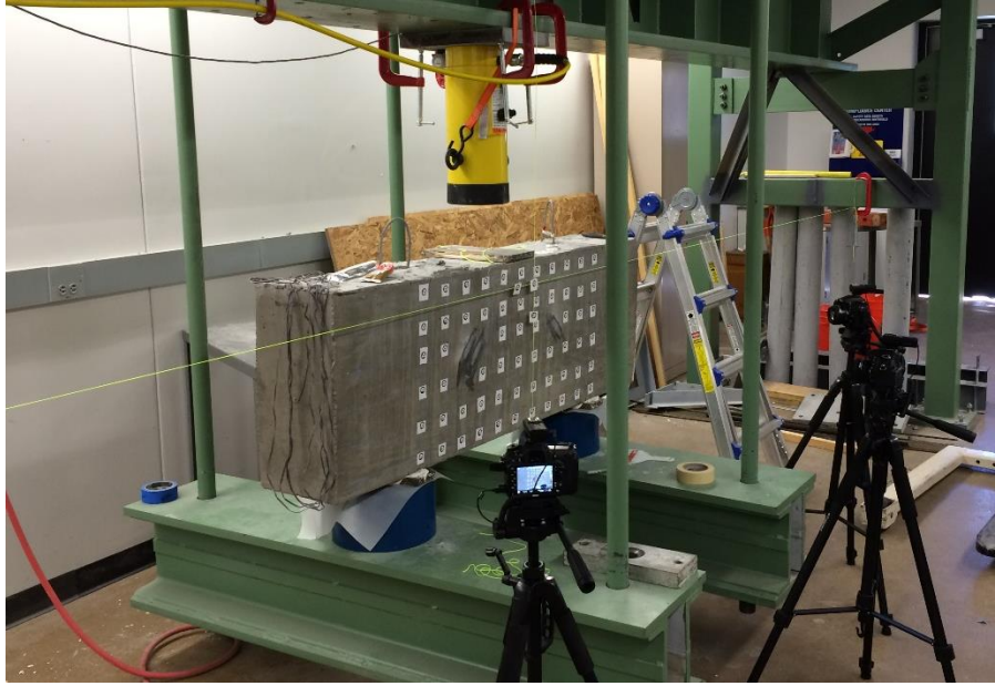
Figure 3-21: Set up of Camera for Photogrammetry
