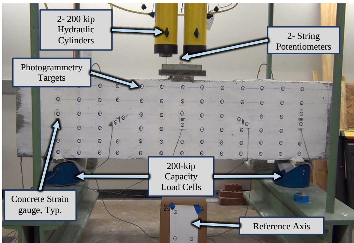
Figure 3-14: Beam Test Setup
