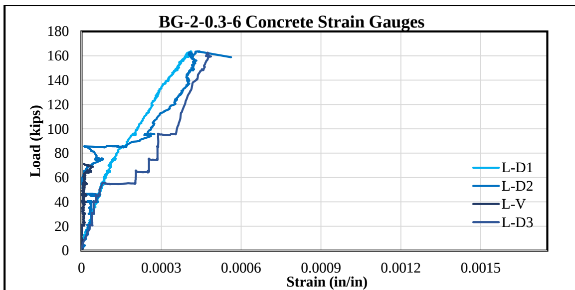
Figure 4-7: Concrete Strain Data for Gauges Shown in Figure 4-6
