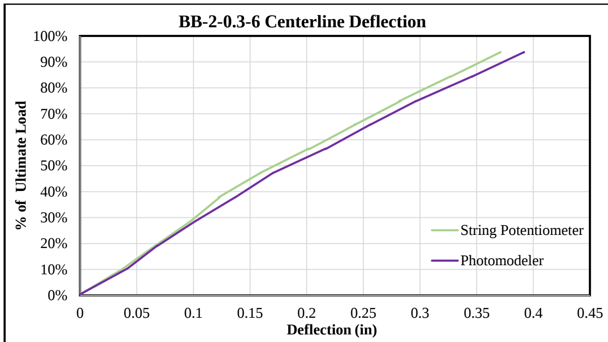
Figure 4-3: Photomodeler vs. String Potentiometer Centerline Deflection on BB-2-0.3-6
