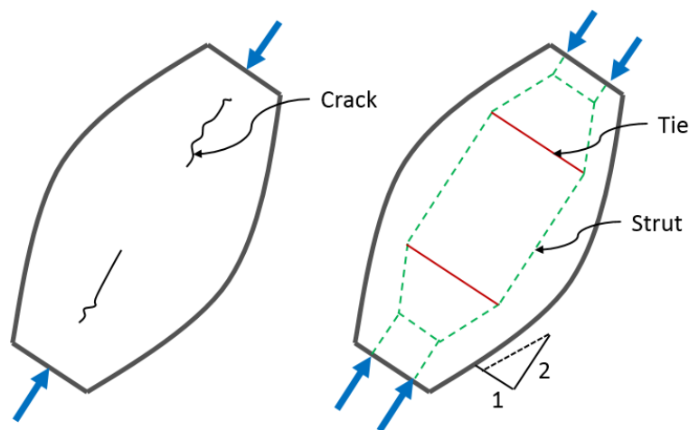
Figure 2-7: Bottle shaped strut adapted from (ACI 318 2014)
