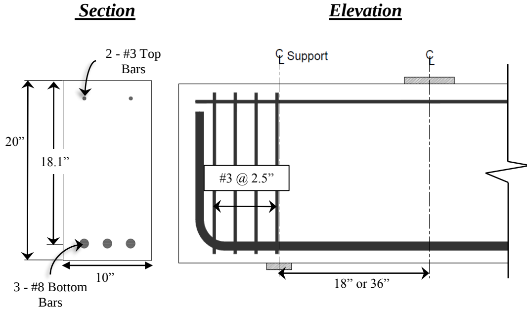
Figure 3-2: Specimens BG-1-0-0 & BG-2-0-0
