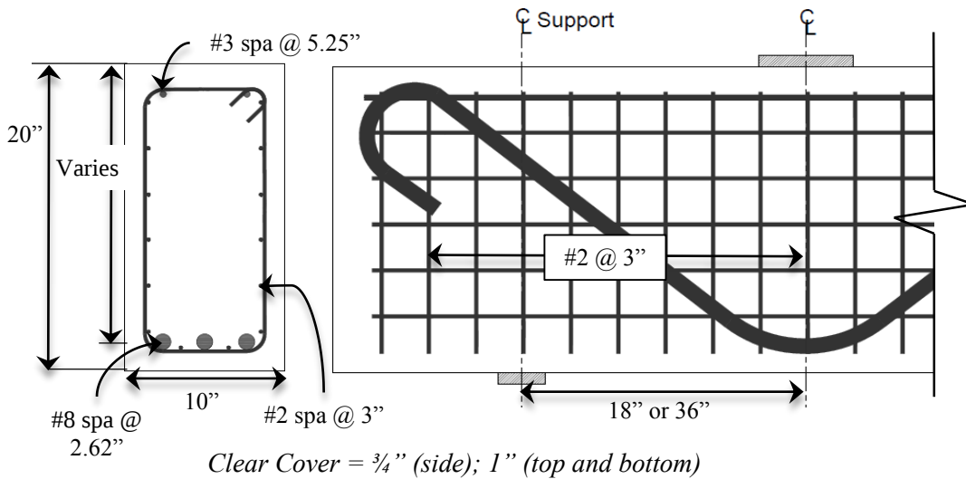
Figure 3-7: Specimens BB-1-0.3-6 & BB-2-0.3-6
