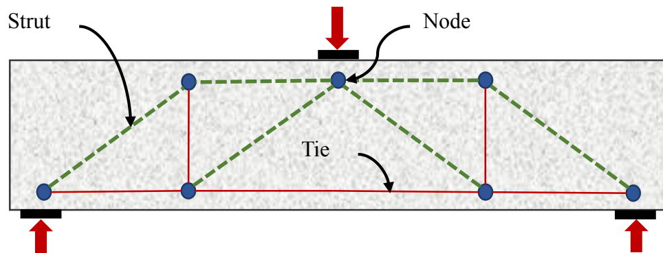
Figure 2-3: Example STM for a point-loaded beam.
