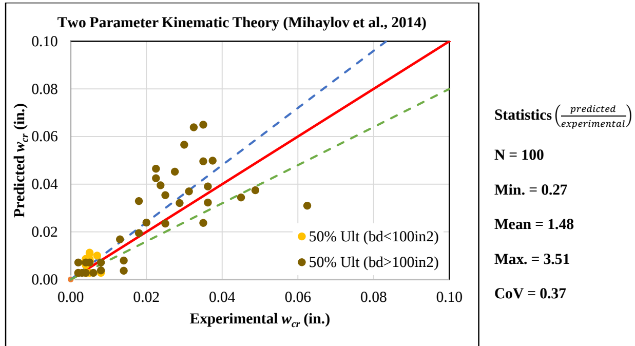
Figure 2-17: Predicted versus experimental crack widths predicted per Mihaylov et al., 2014
