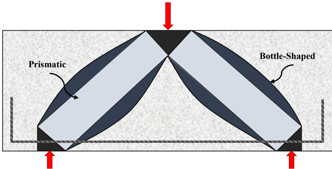
Figure 2-5: STM containing bottle-shaped and prismatic struts
