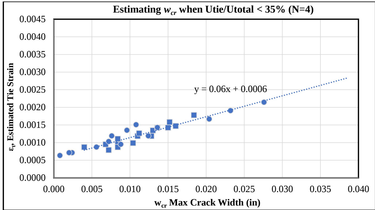
Figure 5-16: Design Tool for Estimating Crack Widths ( \rho = 0.3\% )
