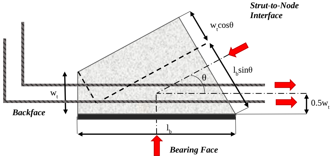
Figure 2-11: CCT Node
