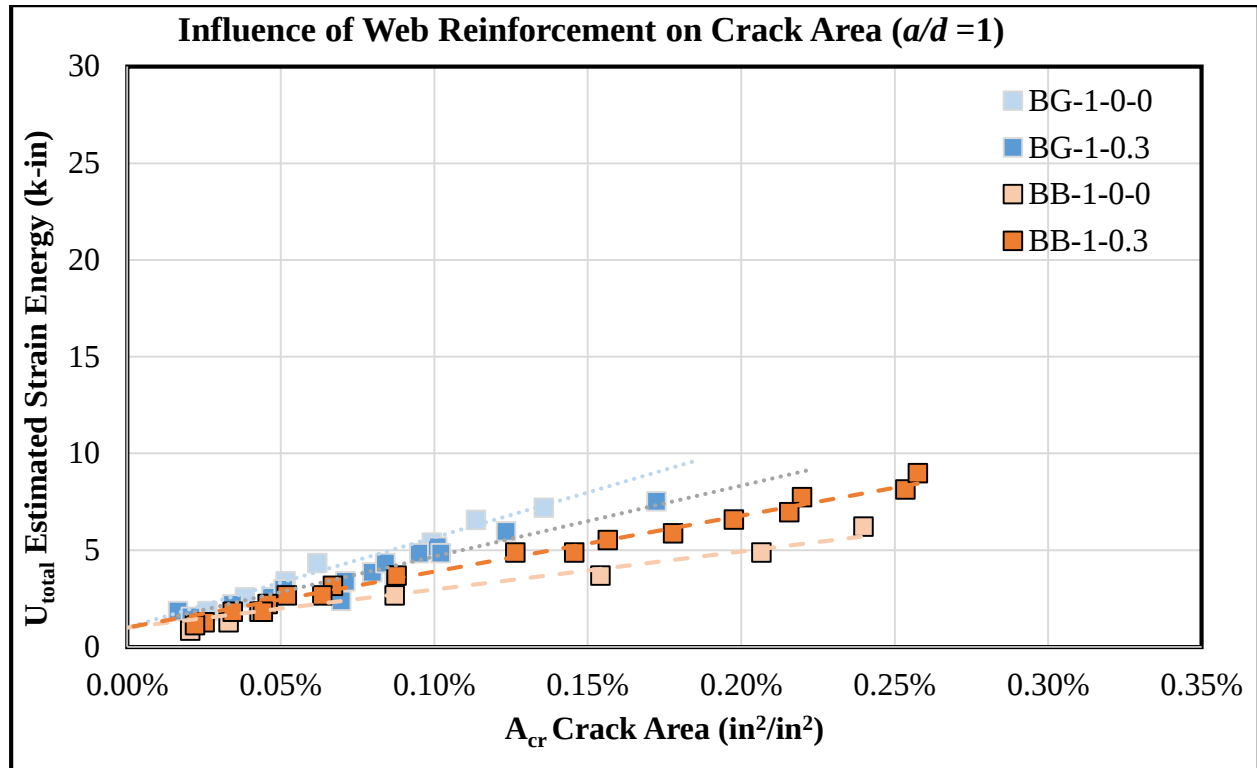
Figure 5-6: Influence of Web Reinforcement on Crack Area ( a/d = 1 )
