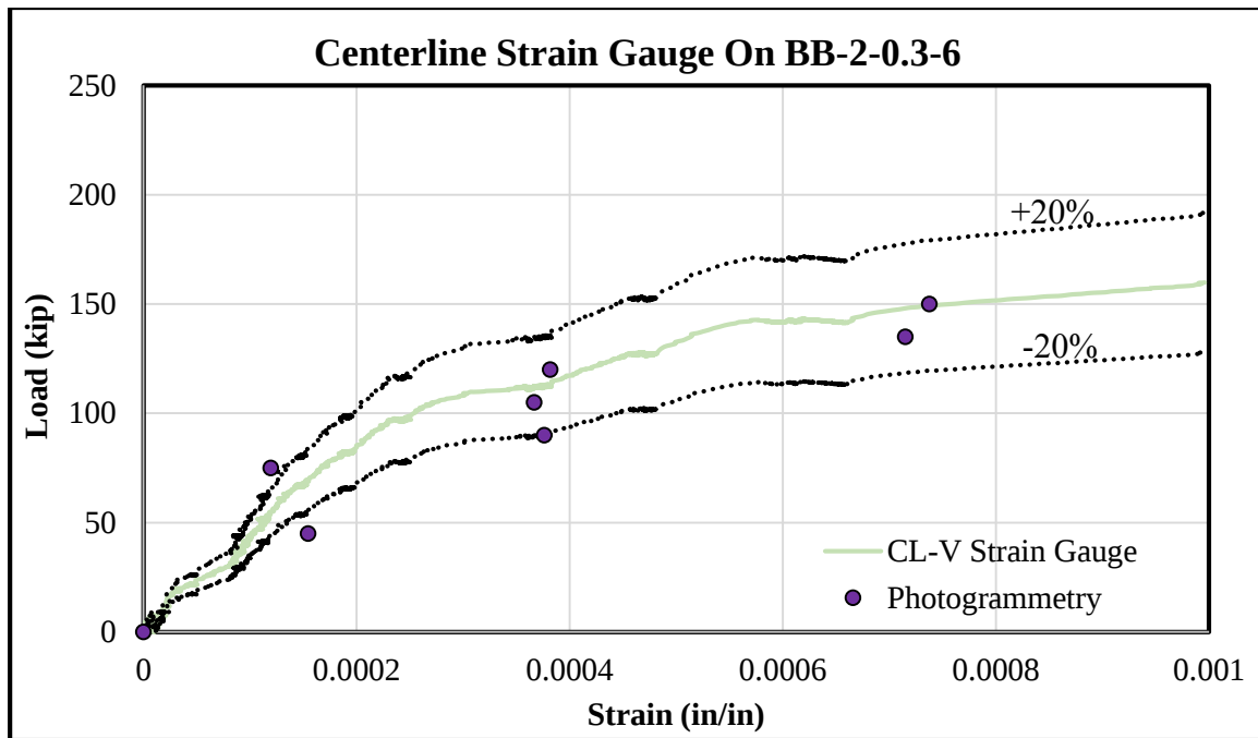
Figure 4-5: Photomodeler vs. Concrete Strain Gauge Data for locations shown in Figure 4-4
