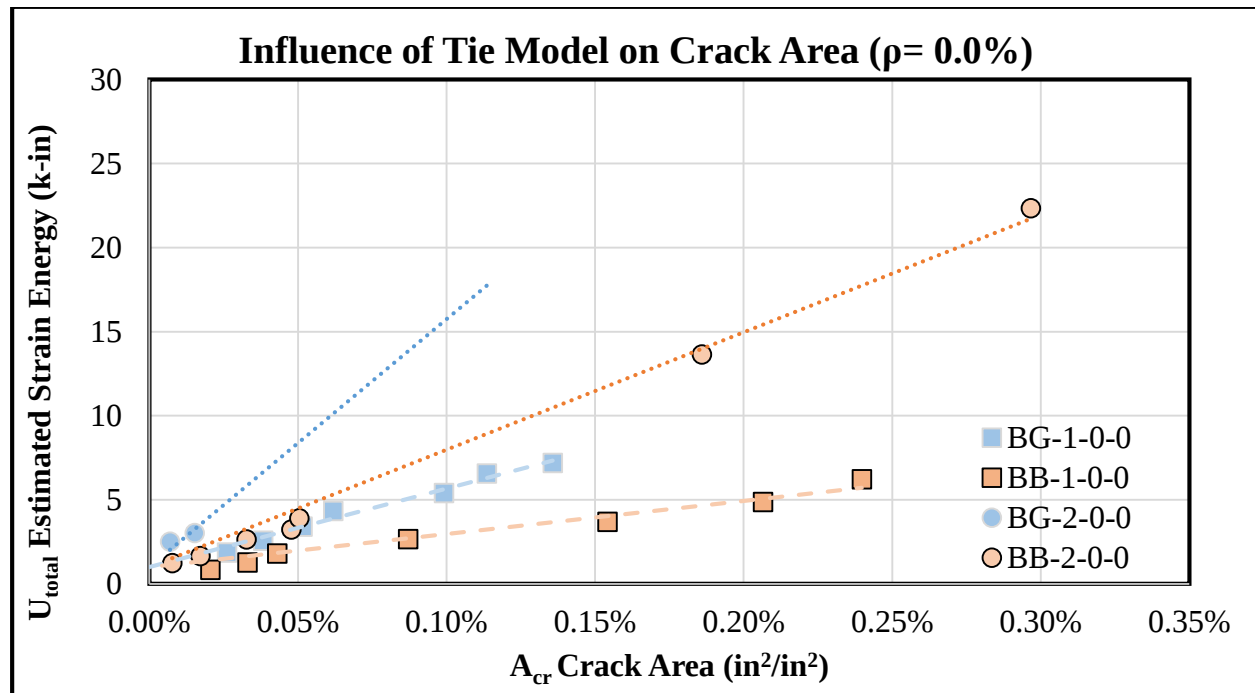
Figure 5-10: Influence of Tie Model on Crack Area ( \rho = 0.0\% )
