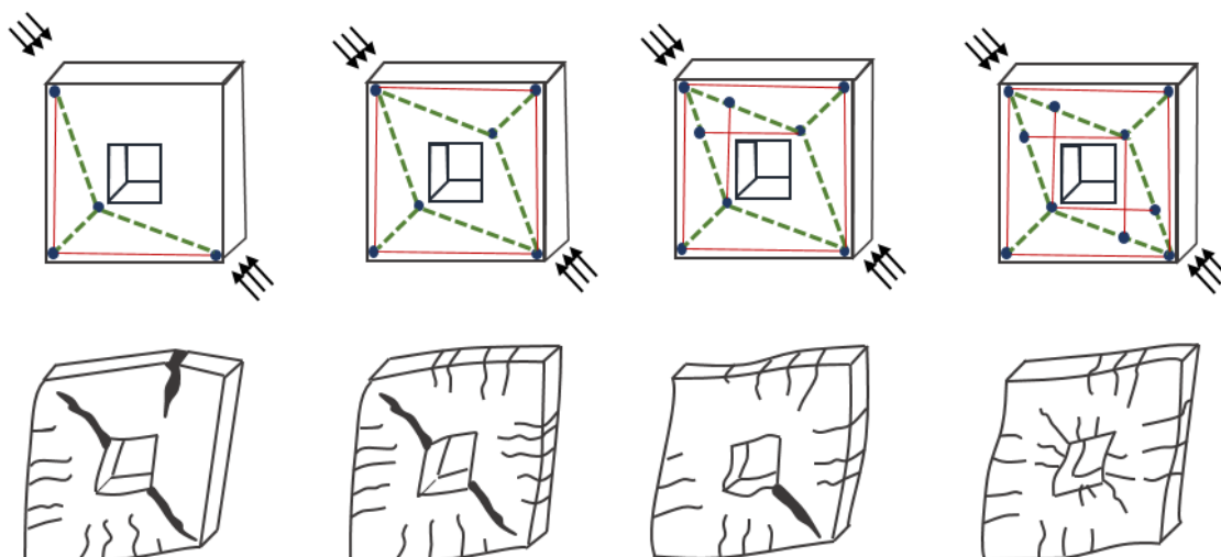
Figure 2-15: Procedure for Designing Suitable Stress Fields (Muttoni et al., 1997)
