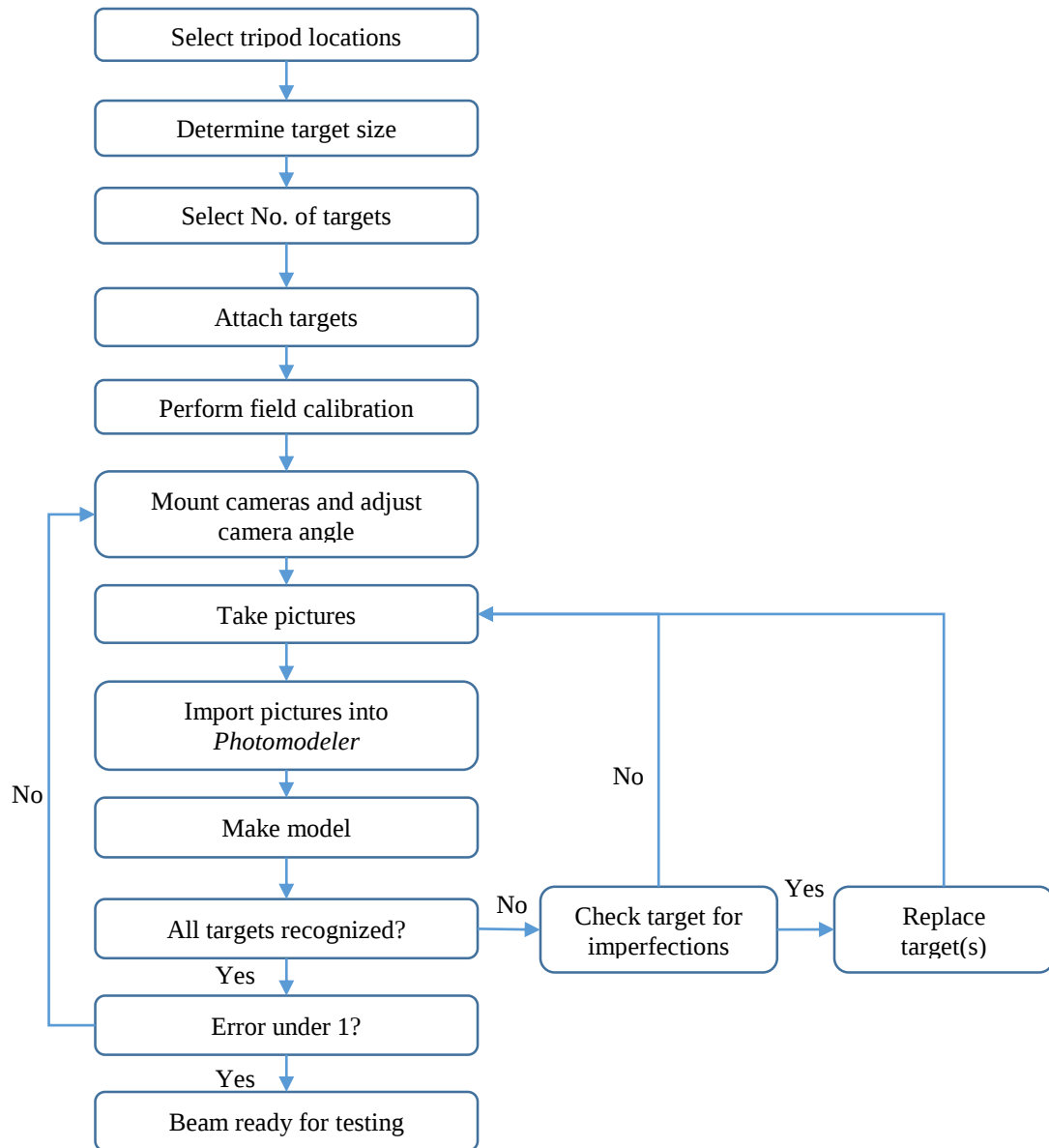
Figure 3-23: Photogrammetry Setup Flowchart
