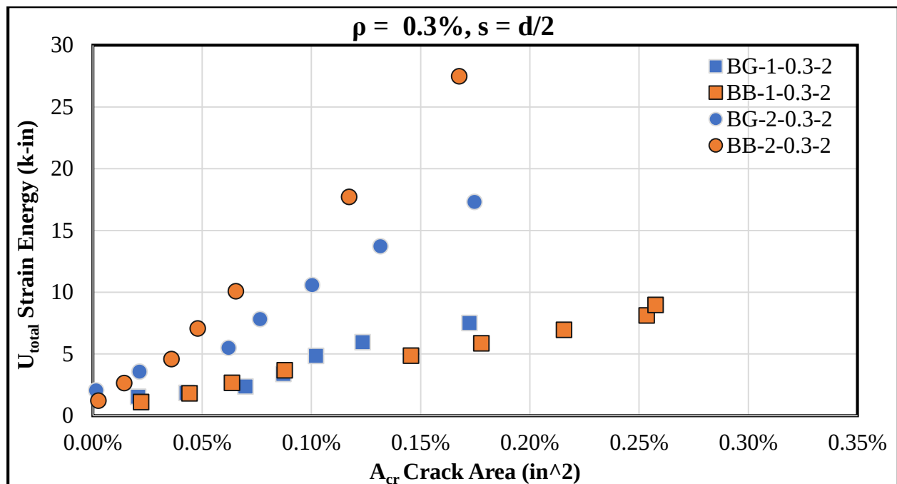
Figure 4-15: Normalized Crack Area vs. Total Strain Energy for \rho = 0.3\% , s = d/2
