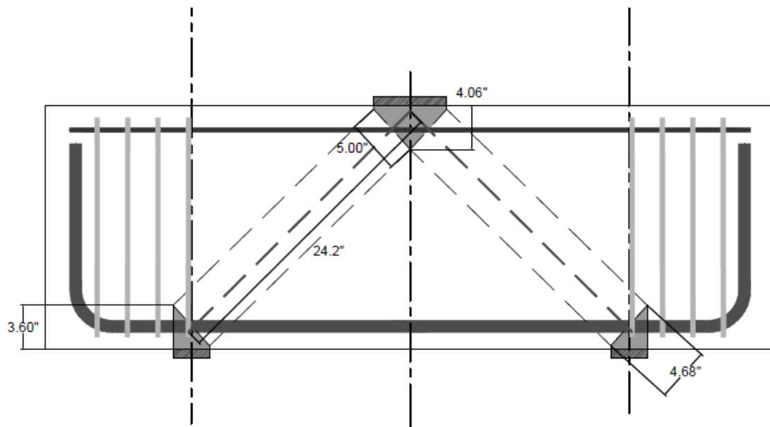
Series 1 Model G Scale 1:10
