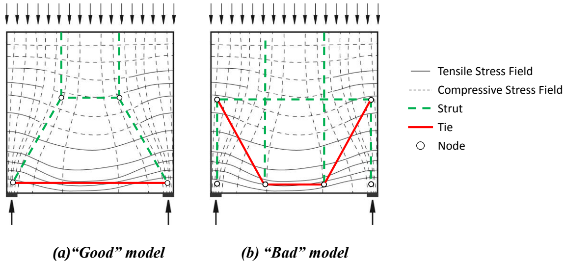
Figure 2-14: Identical structures with force paths represented by a (a) “Good” and (b) “Bad” STM (Schlaich et al, 1987).
