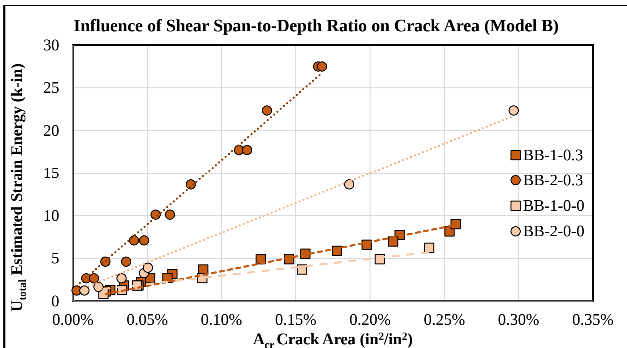
Figure 5-12: Influence of Shear Span-to-Depth Ratio on Crack Area (Model B)
