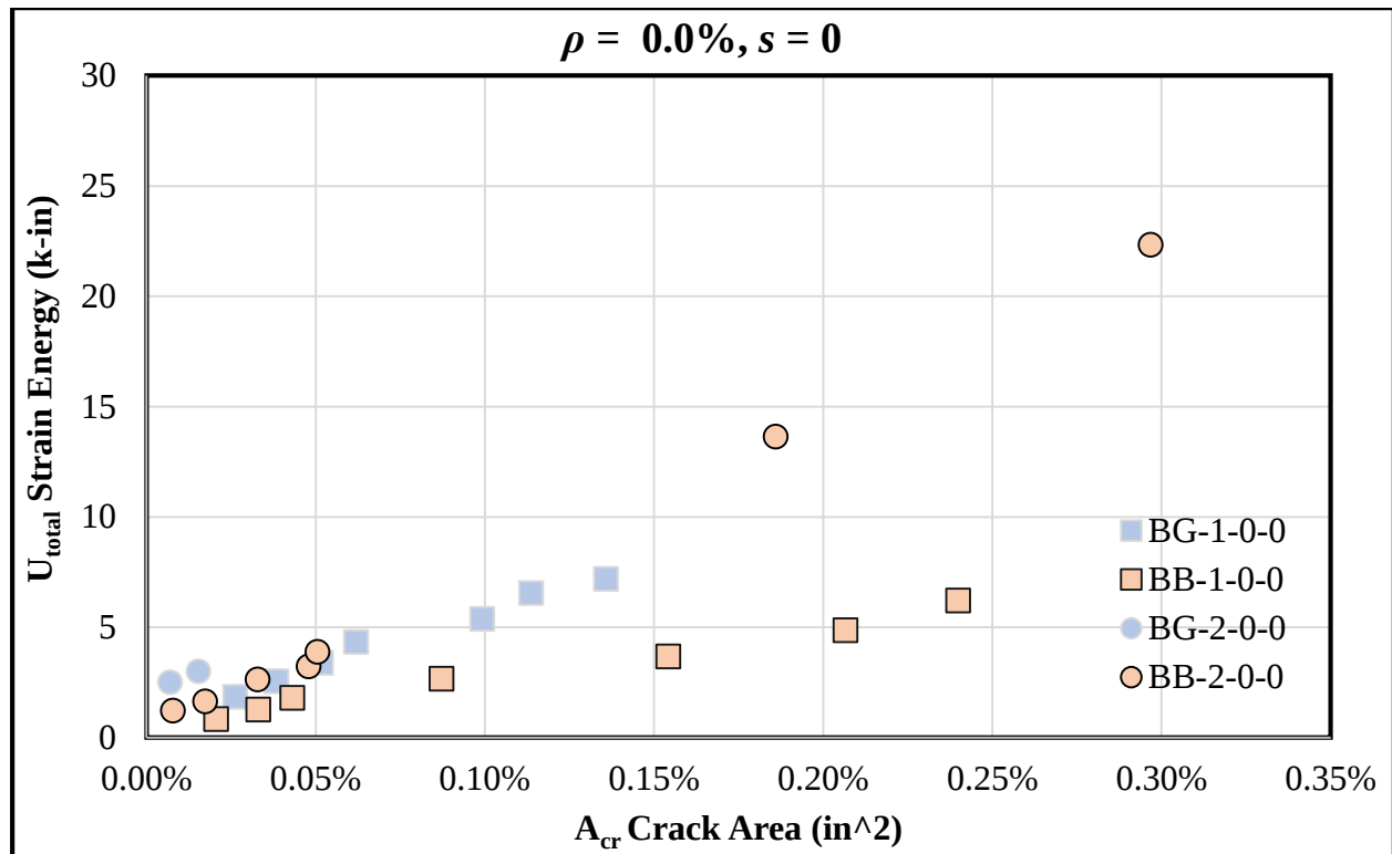
Figure 4-14: Normalized Crack Area vs. Strain Energy for \rho = 0.0\% , s = 0
