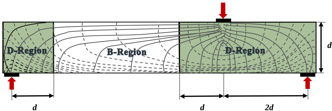
Figure 2-2: Typical concrete beam showing B- and D-regions
