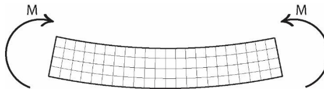
Figure 2-1: Beam theory based on the assumption that planar sections remain planar.
