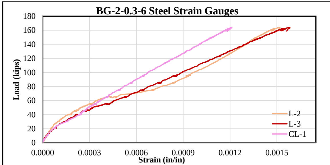
Figure 4-8: Steel Strain Data for Gauges Shown in Figure 4-6.
