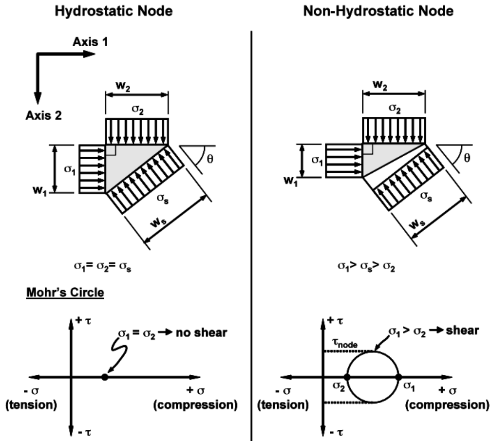
Figure 2-9: Stresses on Hydrostatic and Non-Hydrostatic Nodes (Thompson 2002)
