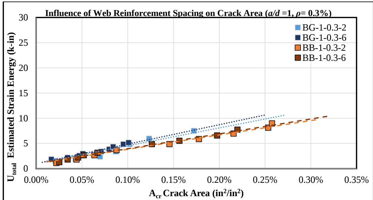
Figure 5-8: Influence of Web Reinforcement Spacing on Crack Area ( a/d = 1, \rho = 0.3\% )
