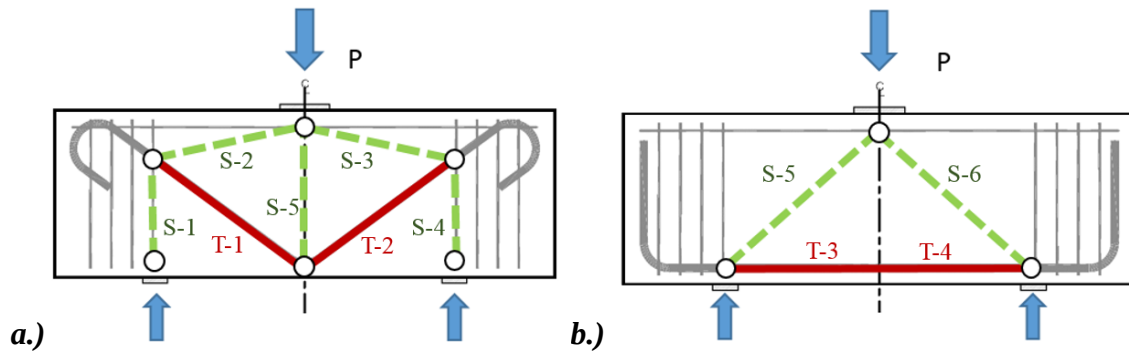
Figure 3-8: Strut and Tie Label Notation for a.) Model B and b.) Model G Beams
