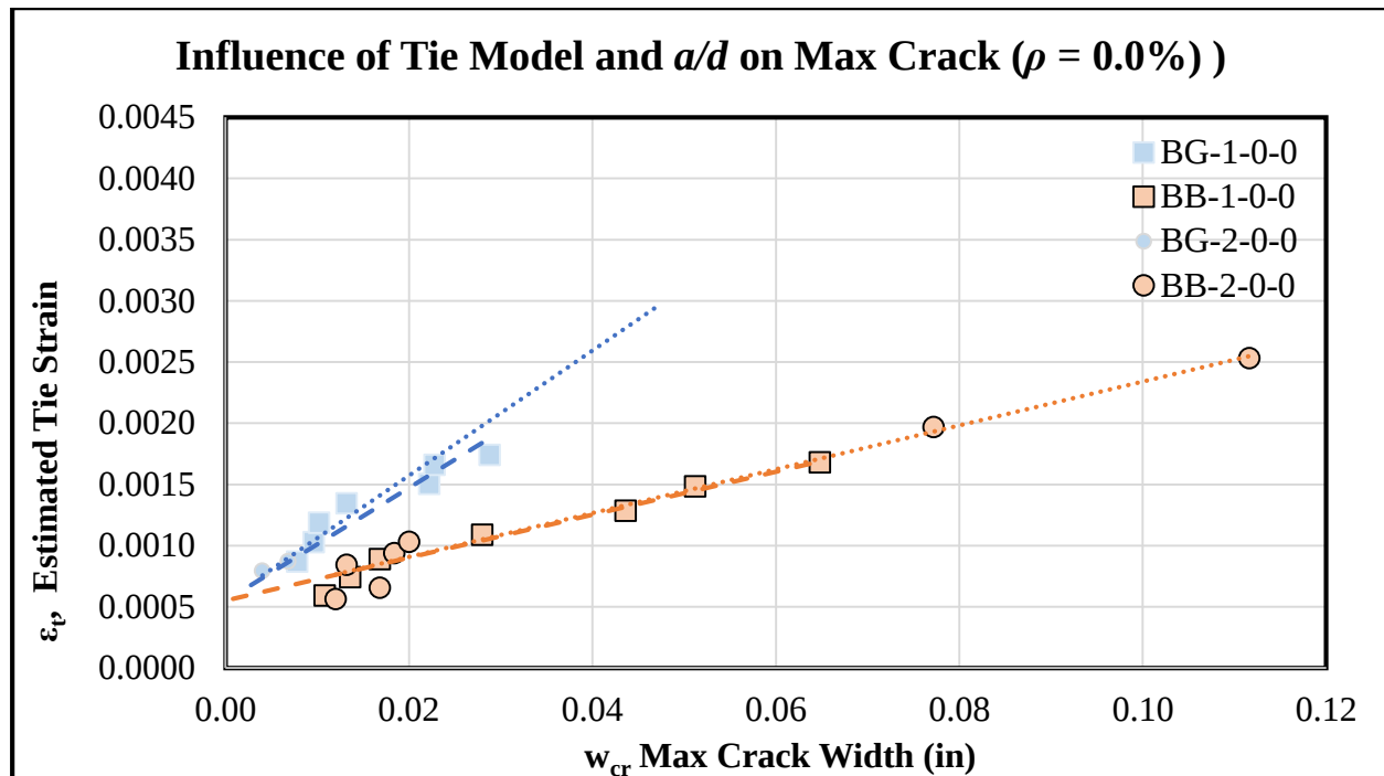
Figure 5-5: Influence of Tie Design on Max Crack ( \rho = 0.0\% )
