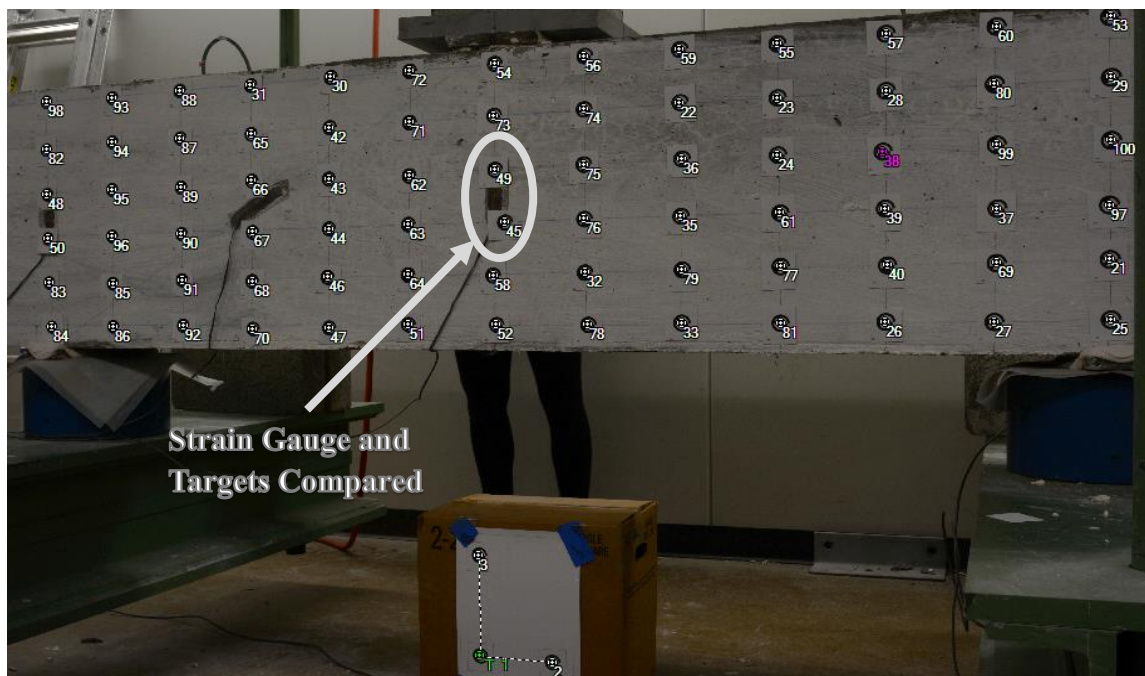
Figure 4-4: Target and Concrete Strain Gauge Location Used for Comparison on BB-2-0.3-6
