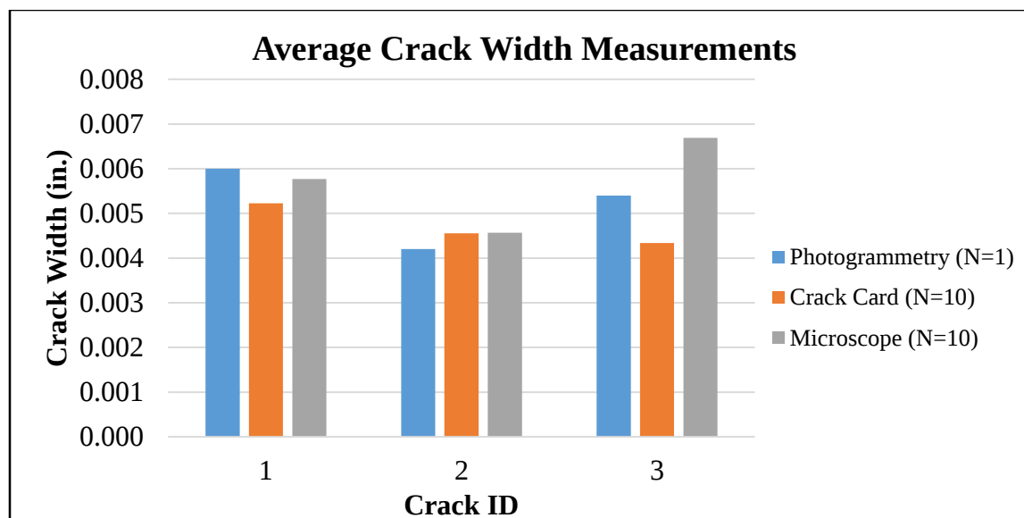
Figure 3-24: Results of Measured Crack Widths Using Three Different Methods
