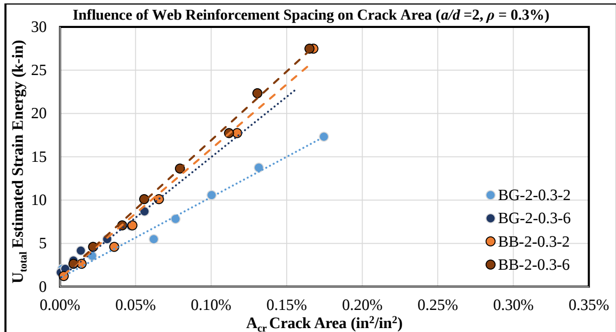
Figure 5-9: Influence of Web Reinforcement Spacing on Crack Area ( a/d = 2, \rho = 0.3\% )
