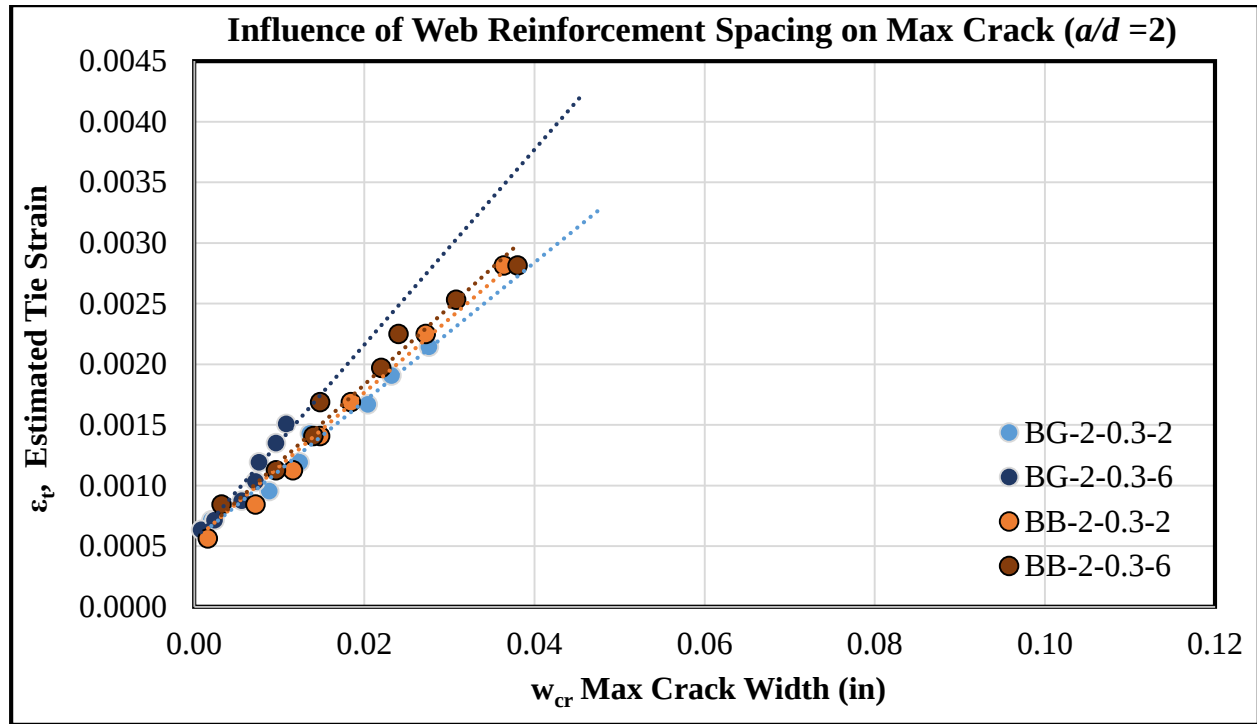
Figure 5-4: Influence of Web Reinforcement Spacing on Max Crack ( a/d = 2 )
