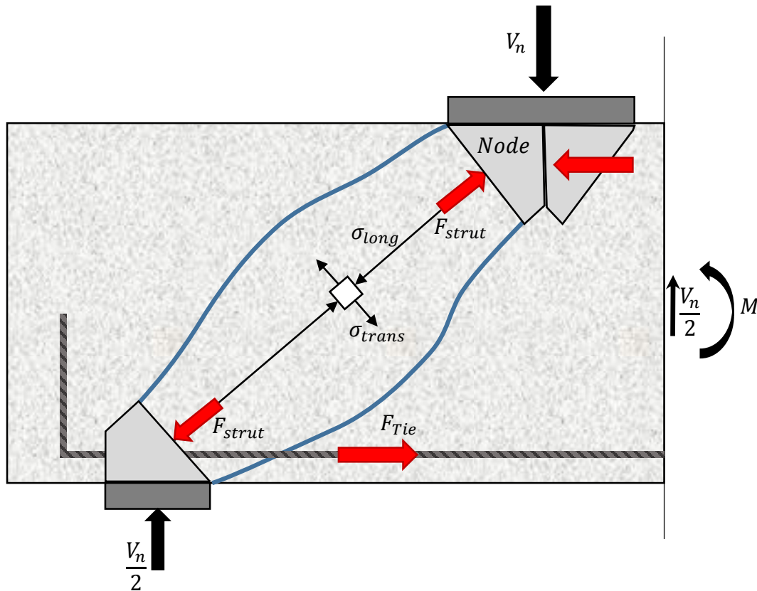
Figure 2-4: Strut and Tie Model shows truss elements and applied internal forces
