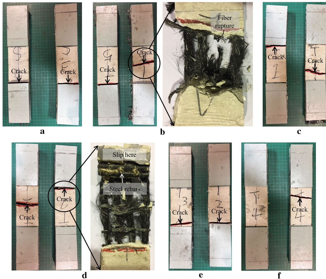
Fig. 6 Failure mode of TRM test specimens in this study. a BASE, b SPREAD, c TAB, d REBAR, e L_COAT, f SL_COAT.
