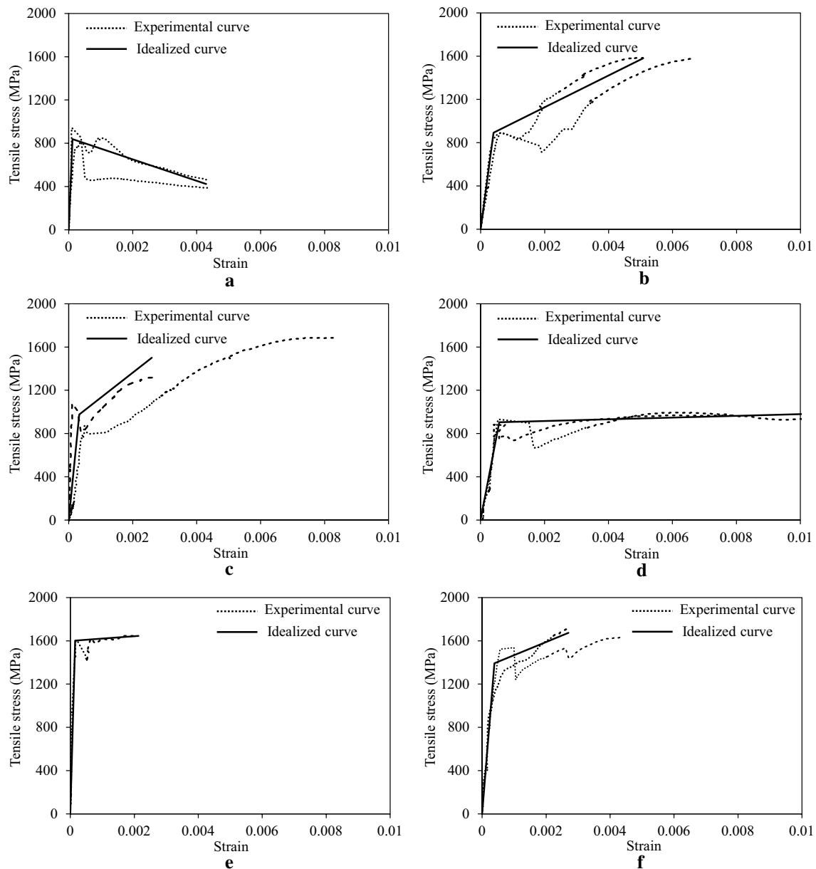
Fig. 11 Idealized and experimental stress–strain curves of TRM test specimens in this study. a BASE, b SPREAD, c TAB, d REBAR, e L_COAT, f SL_COAT.
