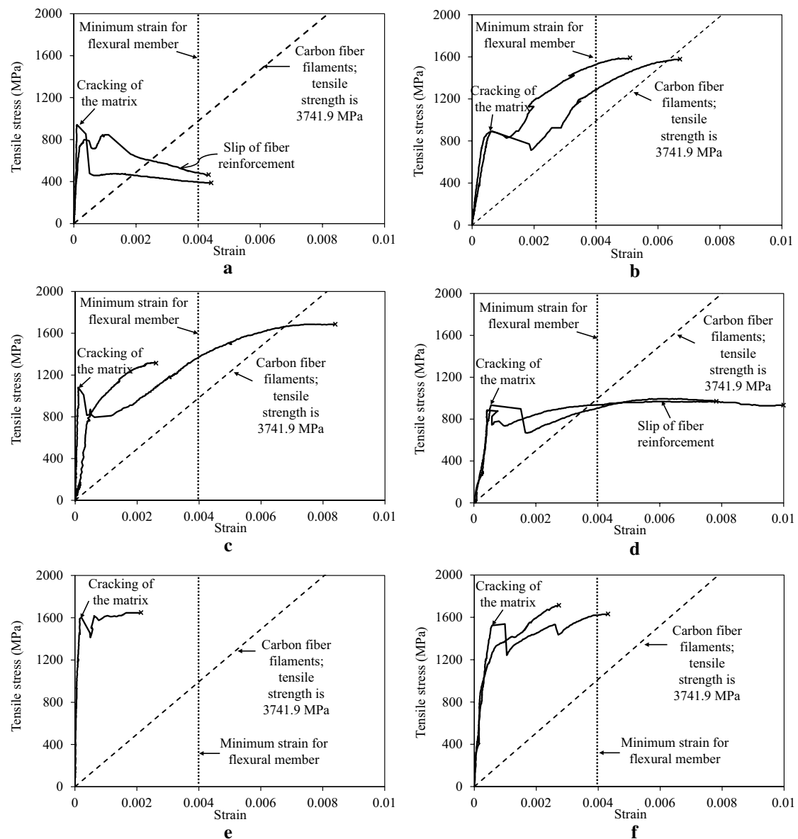
Fig. 7 Stress-strain relationship of test specimens. a BASE, b SPREAD, c TAB, d REBAR, e L_COAT, f SL_COAT.
