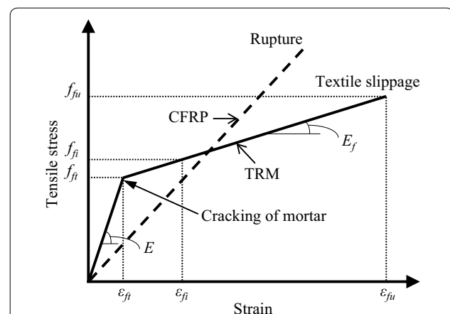
Fig. 10 Idealized stress–strain curve of TRM test specimen according to ACI 549.4R-13 (2013).
