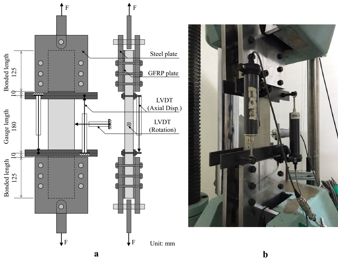
Fig. 4 Tensile test setup. a Scheme of test setup, b Photo of test setup.
