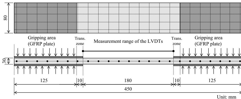
Fig. 2 Typical details of test specimens.
