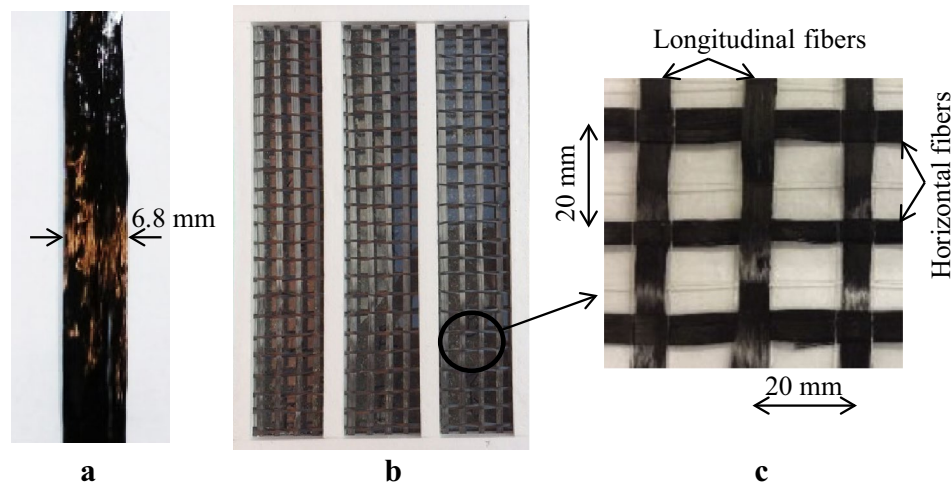
Fig. 1 Details of carbon fiber mesh used as textile reinforcement. a Carbon fiber filament provided by manufacturer, b Carbon fiber mesh, c Geometrical dimensions.
