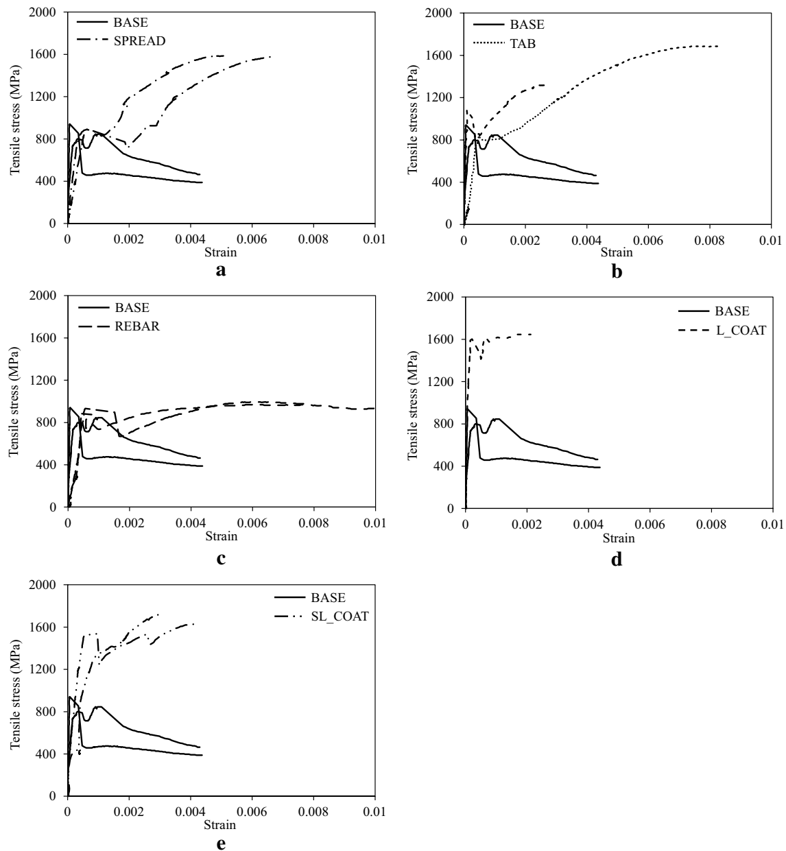
Fig. 8 Effect of anchorage methods on tensile behaviors of test specimens. a Effect of SPREAD method, b Effect of TAB method, c Effect of REBAR method, d Effect of L_COAT method, e Effect of SL_COAT method
