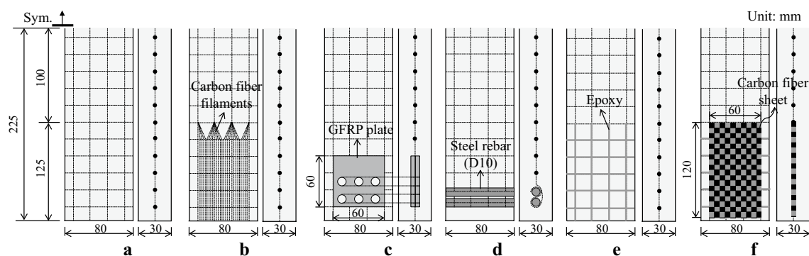
Fig. 3 Details of anchorage methods. a BASE, b SPREAD, c TAB, d REBAR, e L_COAT, f SL_COAT.
