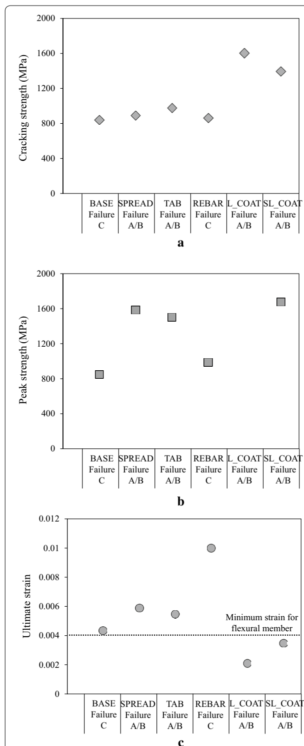
Fig. 9 Comparison of average cracking strength, average peak strength and average ultimate strain of TRM test specimens. a Effect of anchorage methods on cracking strength, b Effect of anchorage methods on peak strength, c Effect of anchorage methods on ultimate strain.
