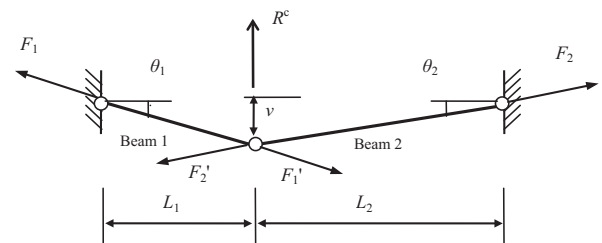
Fig. 13 Schematic diagram of catenary mechanism of beams.
