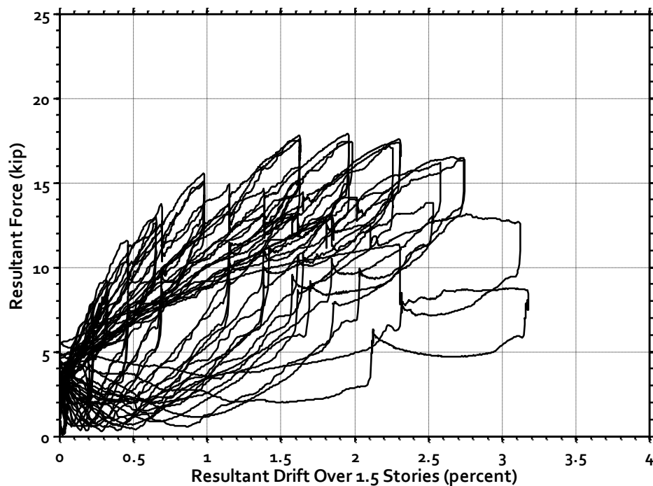
Figure 3-26: Specimen B1 – Resultant Load versus Drift Response
