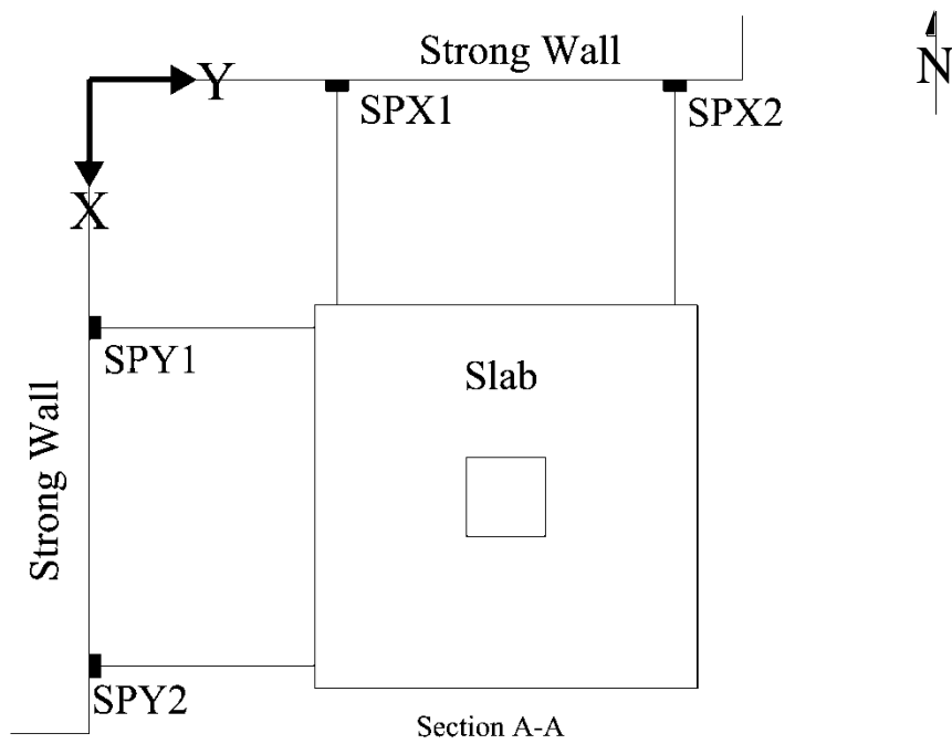
Figure 2-26: String Potentiometer Locations
