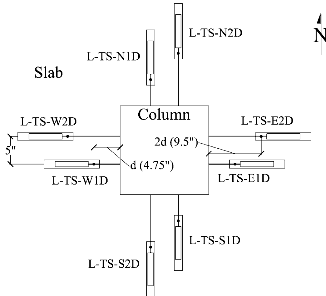
Figure 3-24: LVDT Locations in Slab Region
