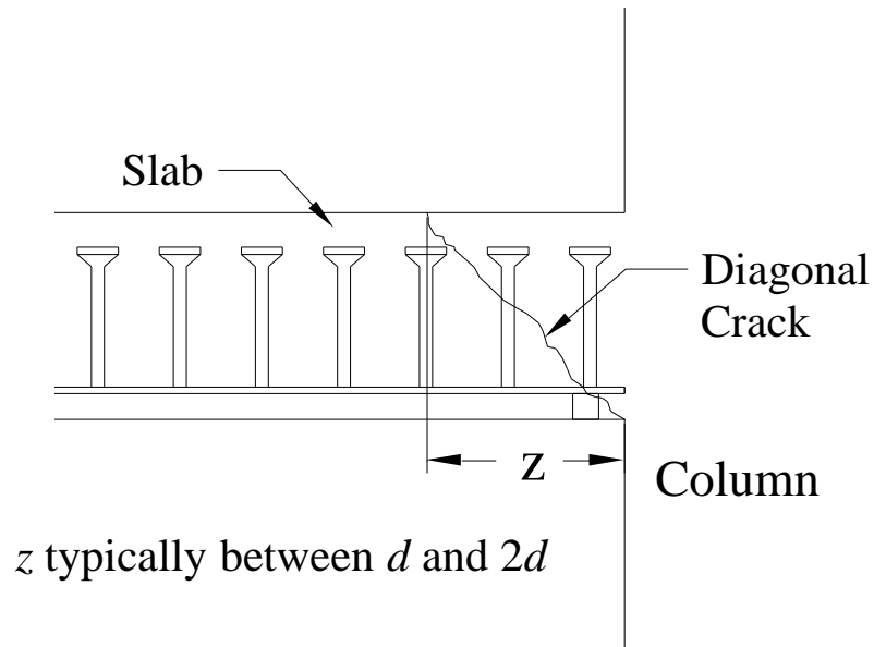
Figure 1-3: Shear Stud Reinforcement Shear Transfer Mechanism
