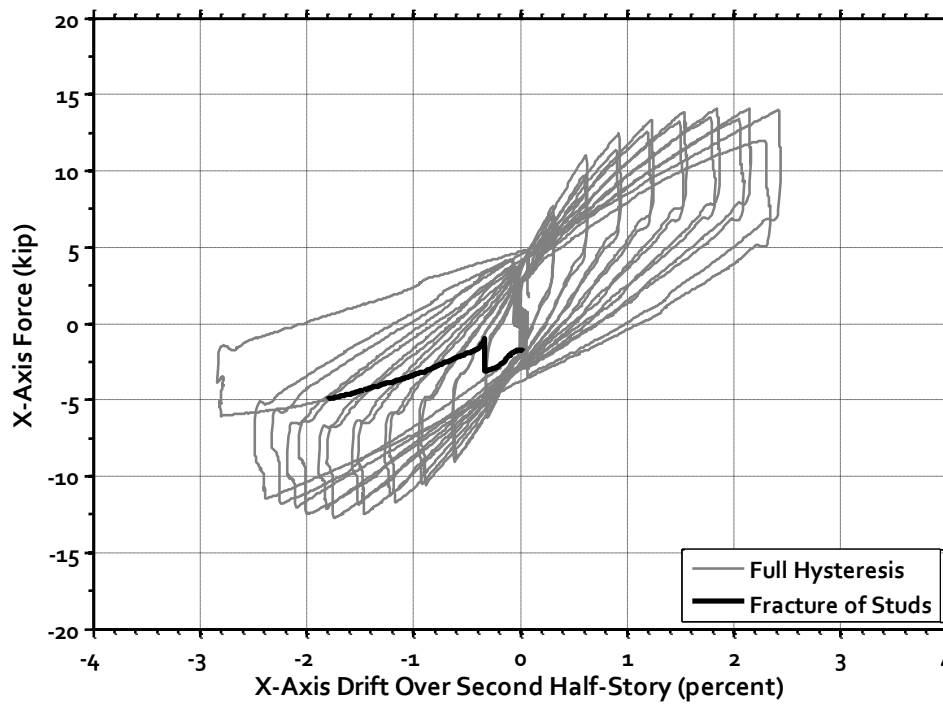
Figure C-6: Specimen B2 – Load versus Second Half-Story Drift in X-Direction
