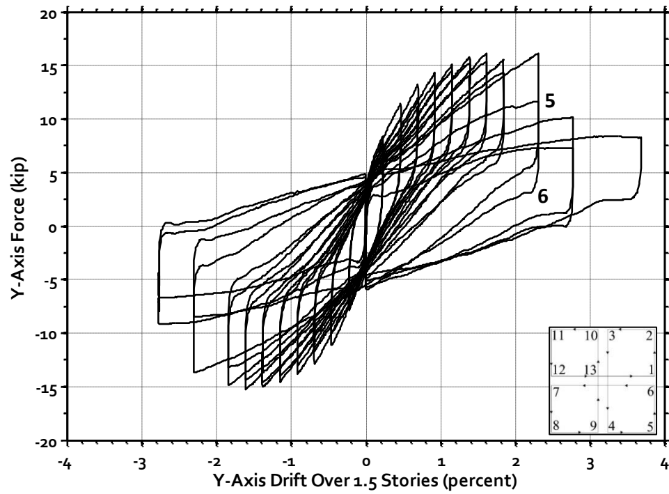
Figure 3-40: Specimen B4 – Load versus Drift Response (Y-Direction)
