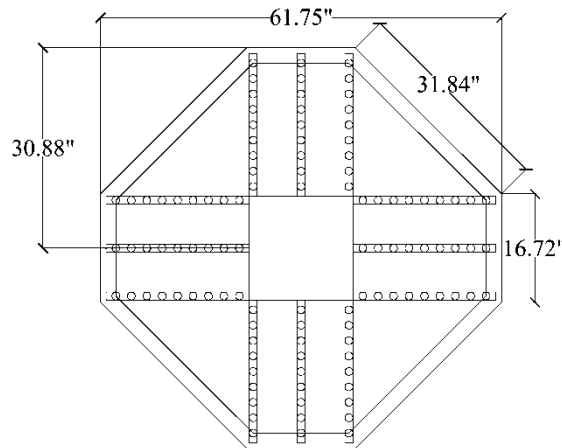
Figure A-1: Shear Reinforcement Layout for Specimen B1
