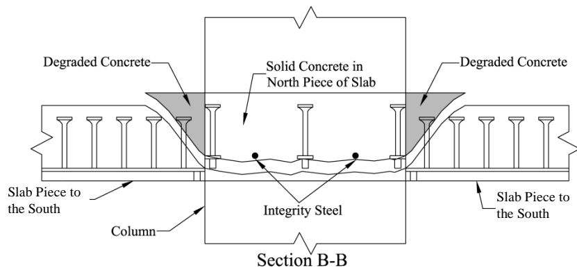
Figure 3-11: Failure Surface of Connection B1
