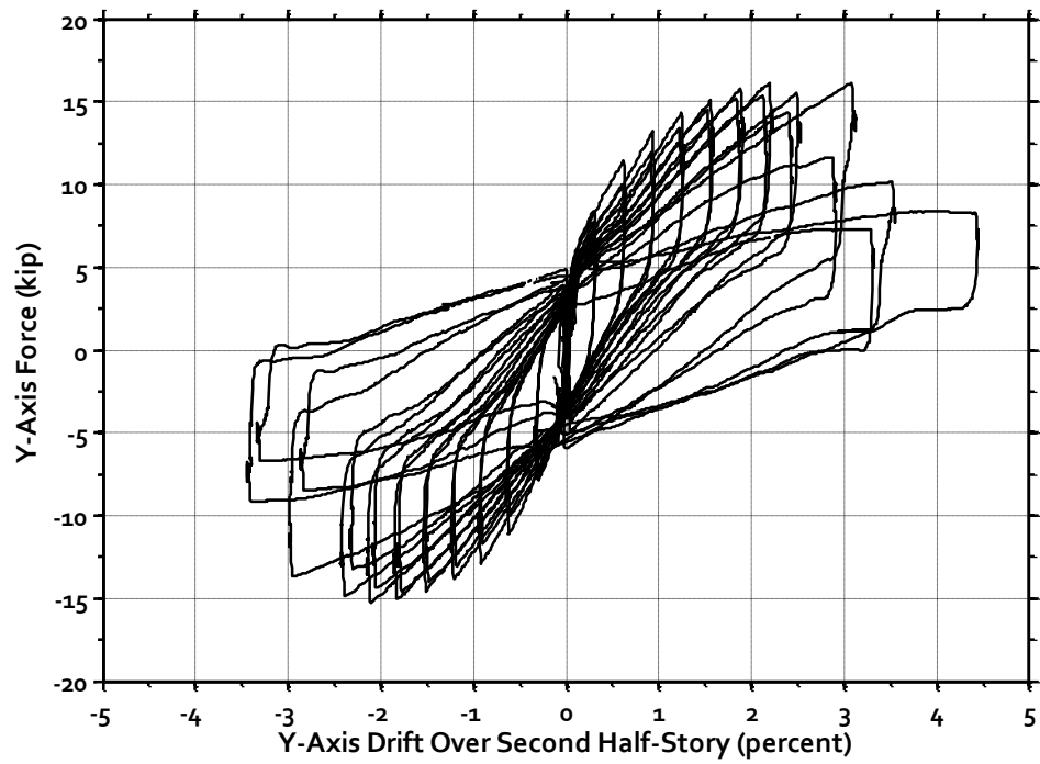
Figure C-16: Specimen B4 – Load versus Second Half-Story Drift in Y-Direction
