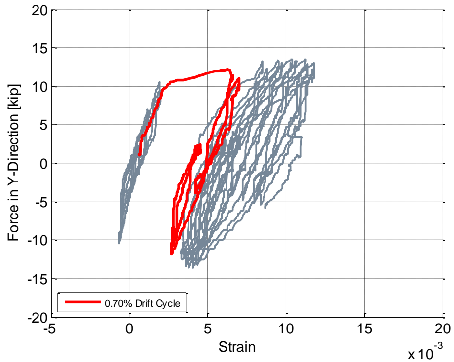
Figure 3-74: Specimen B2 – Lateral Force versus Strain in Gauge TE3
