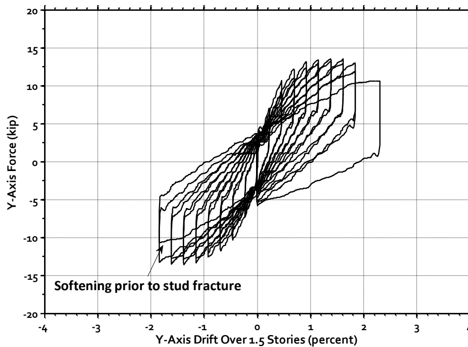
Figure 3-30: Specimen B2 – Load versus Drift Response (Y-Direction)
