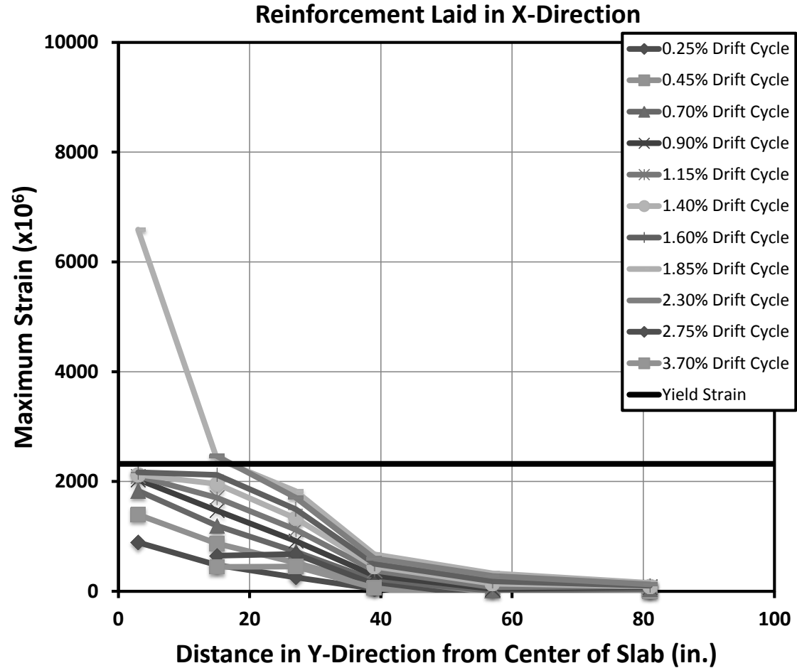
Figure 3-91: Specimen B4 – Profile of Strains in Top Mat Flexural Reinforcement Placed in the X-Direction at d/2 from Column Face. Gauge TS3, Located 3 in. From the Centerline of the Slab, was Damaged After the 1.85% Drift Cycle.
