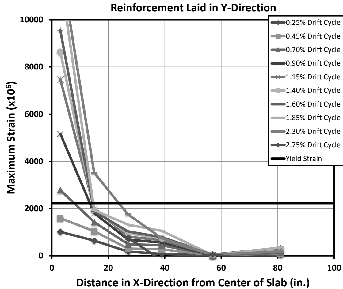
Figure 3-84: Specimen B3 – Profile of Strains in Top Mat Flexural Reinforcement Placed in the Y-Direction at d/2 from Column Face
