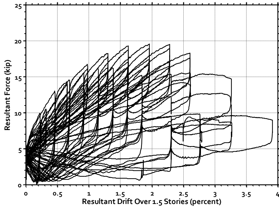
Figure 3-36: Specimen B3 – Resultant Load versus Drift Response
