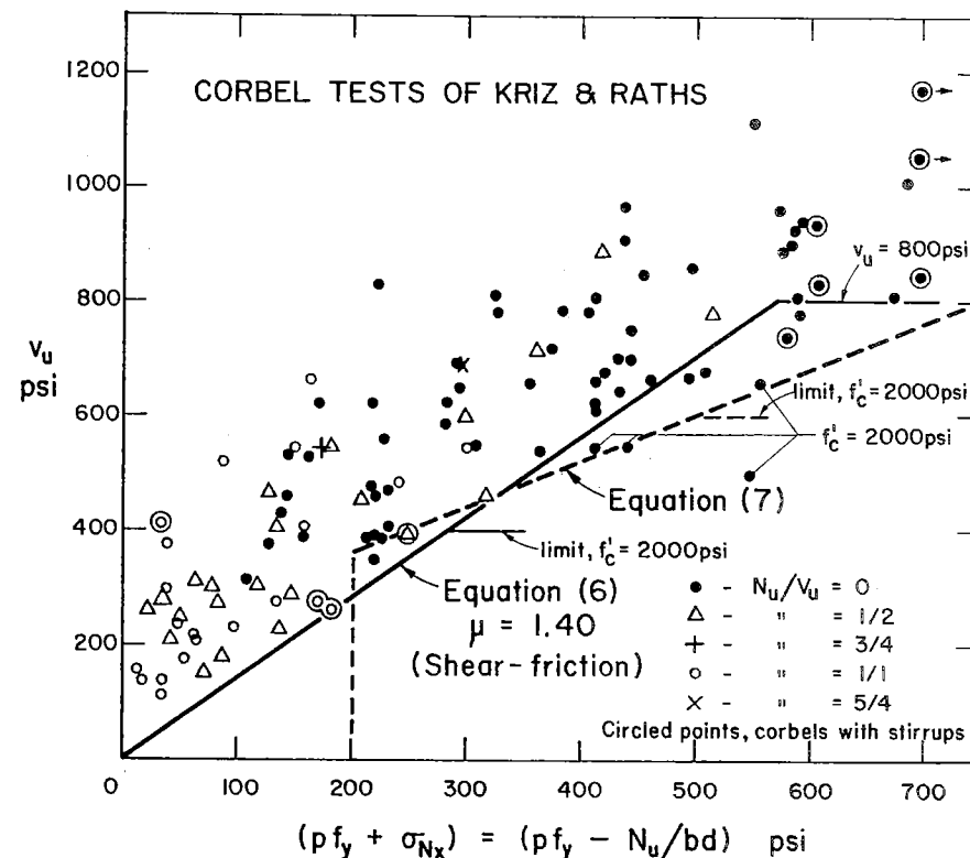
Fig. 12. Comparison of the shear strength of corbels calculated using Eqs. (6) and (7) with the measured strengths of tested corbels
