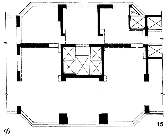
Fig. 9—Shearwall open tube connecting elements: (a) tenth floor; (b) eleventh floor; (c) twelfth floor; (d) thirteenth floor; (e) fourteen floor; (f) fifteenth floor
