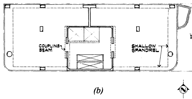
Fig. 1—211 Madison Ave. (recipient of the Concrete Industry Board's 1984 Residential Award): (a) south elevation; (b) typical floor plan (Photo: G. Gwertzman)
