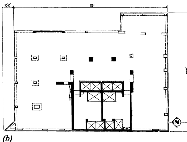
Fig. 6—Metropolitan Tower: (a) typical office level; (b) typical residential level
