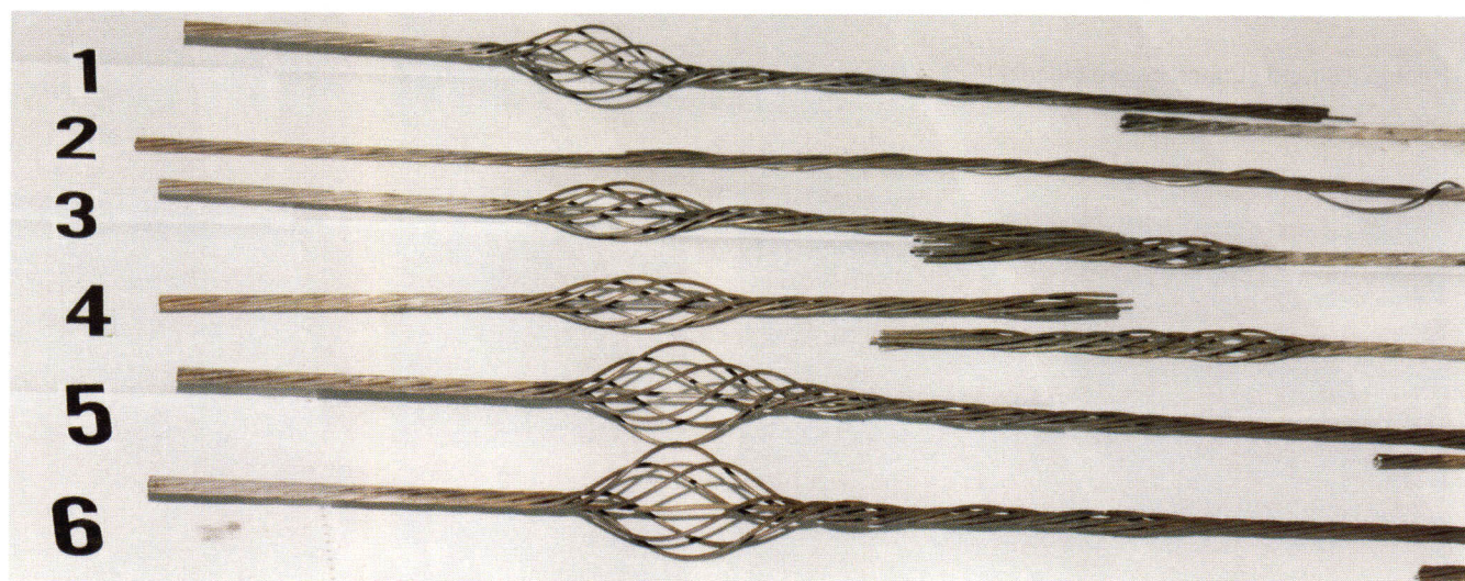
Photo 10. Samples after testing for mechanical properties.
