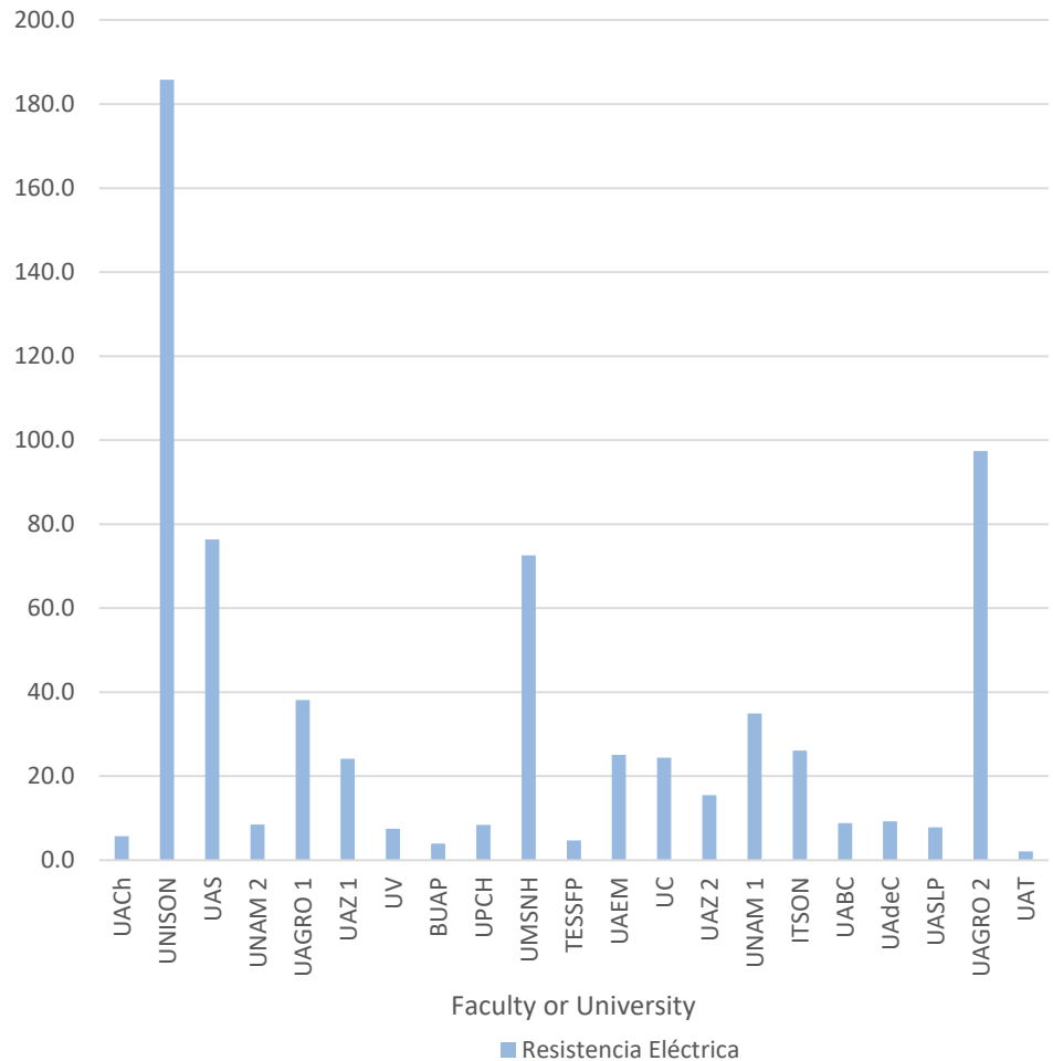
Electric Resistivity
