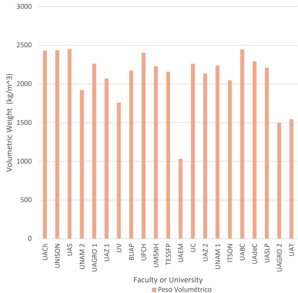
Volumetric Weight
