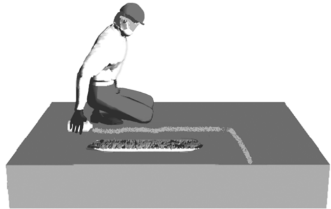
Fig. 2—Mark the perimeter of the repair area using simple geometric shapes and minimizing re-entrant corners.
