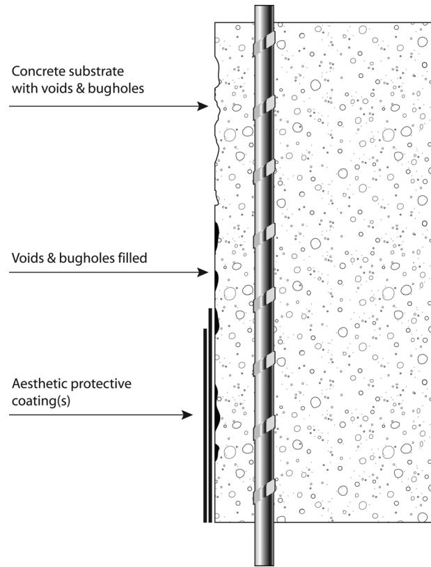
Fig. 1—Through-wall section of a typical concrete surface to be leveled or profiled.
