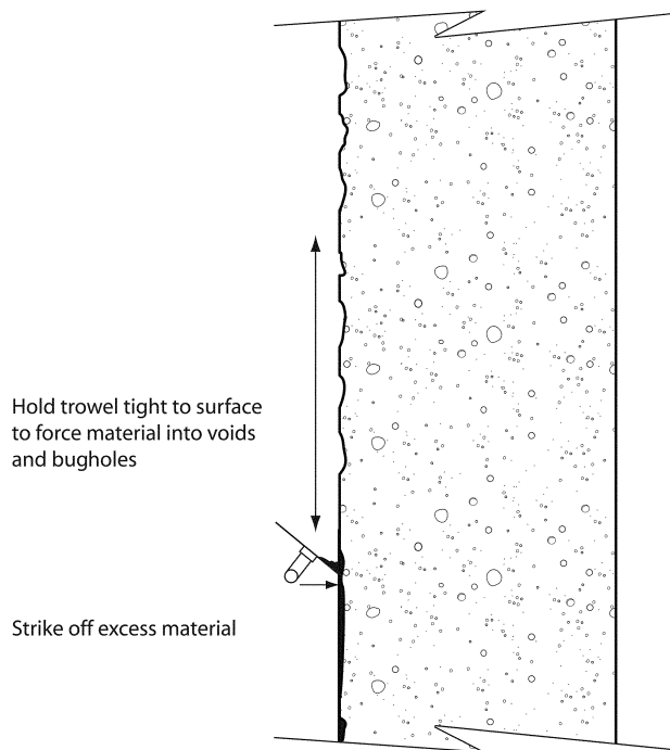
Fig. 4—Troweling material.
