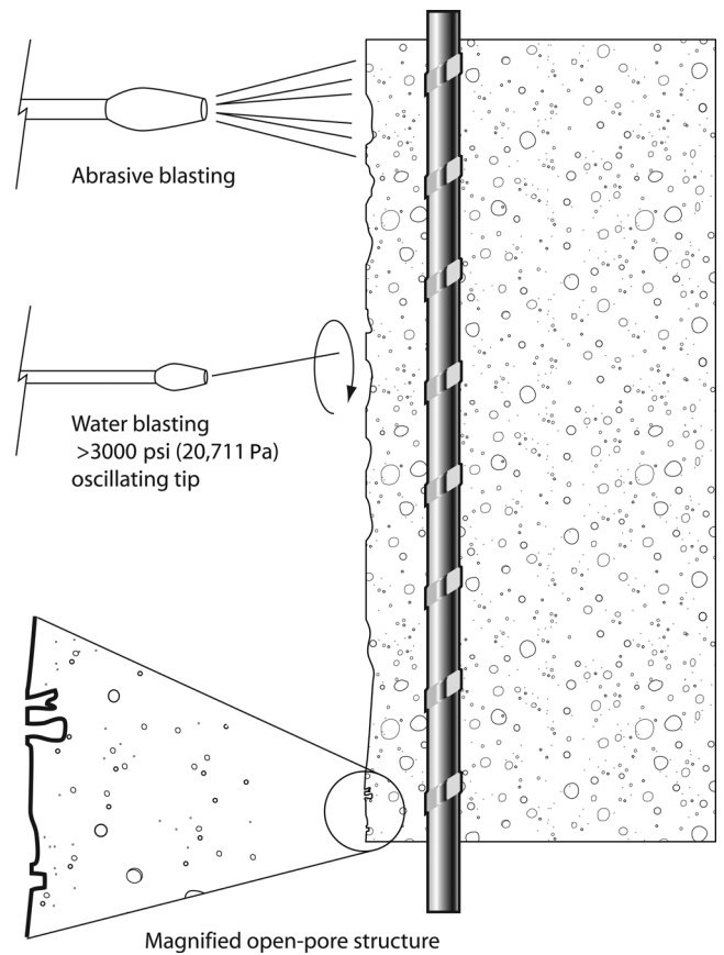
Fig. 3—Surface preparation.
