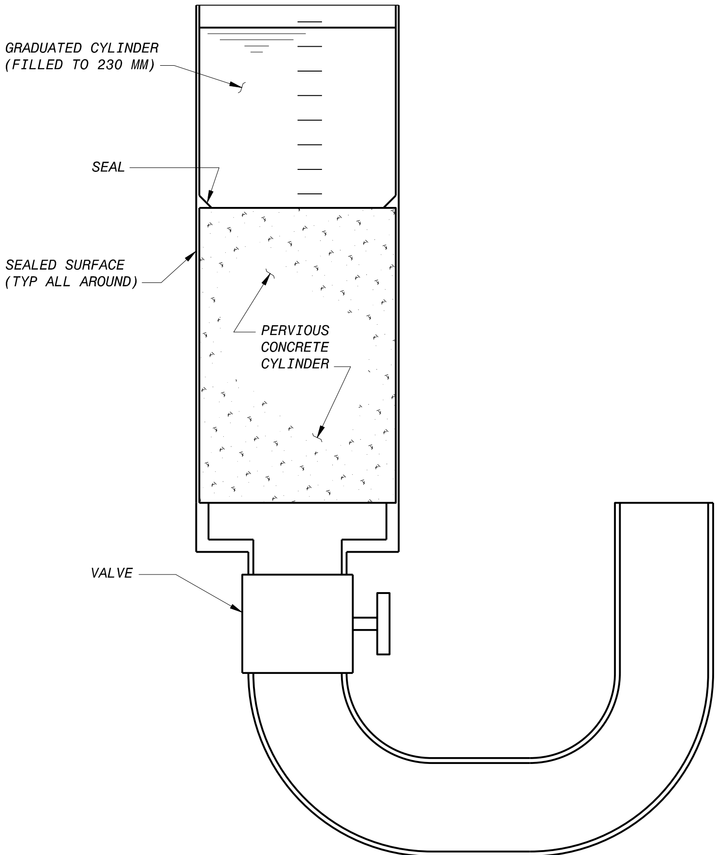
FIGURE 1 - PERMEABILITY TEST SETUP
