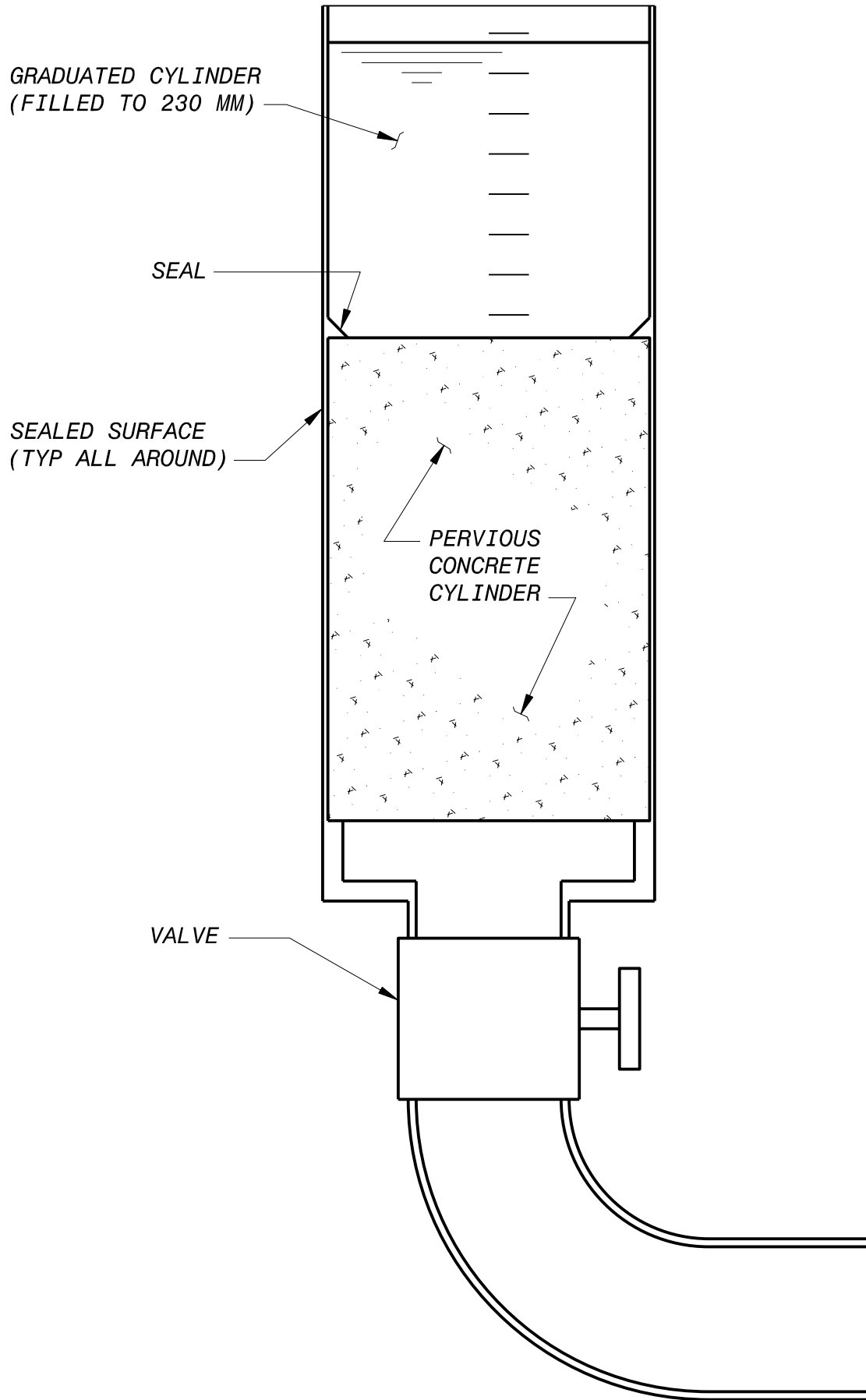
FIGURE 1 - PERMEABILITY TEST SETUP
