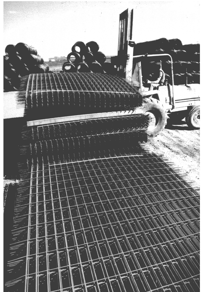
Fig. 3.1.3—Welded wire reinforcement sheets (courtesy of Wire Reinforcement Institute).
